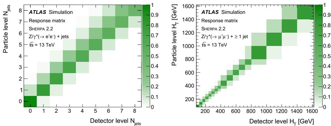
Fig. 2 Response matrices corresponding to the exclusive jet multiplicity for Z + \text{jets} events in the electron channel (left) and to the H_T for Z + \geq 1 jet events in the muon channel (right). The sum of the entries in each row is normalised to unity. Both matrices are obtained from SHERPA 2.2
