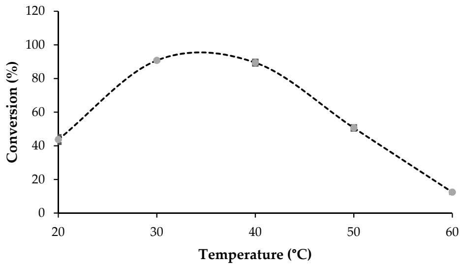
Figure 2. Esterification of OA and 1-octanol at different reaction temperatures. Reaction conditions: 1 mmol of OA, 2mmol of 1-octanol, 1 mL n-heptane, 5 h, and 10% of biocatalyst based on OA mass.
