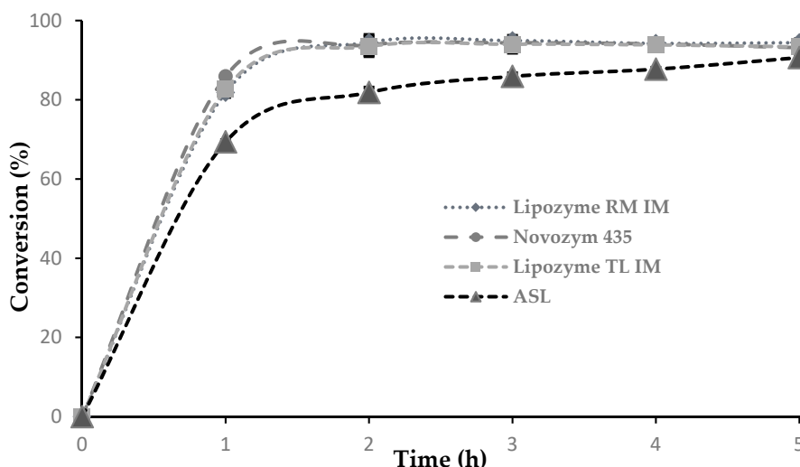
Figure 6. Esterification of OA and 1-pentanol using different biocatalyst. Reaction conditions: 1 mmol of OA, 2 mmol of 1-pentanol, 1 mL n-heptane, 15% of biocatalyst based on OA mass, and 30 °C. Biocatalyst: ASL, Novozym 435, Lipozyme RM IM, Lipozyme TL IM.
