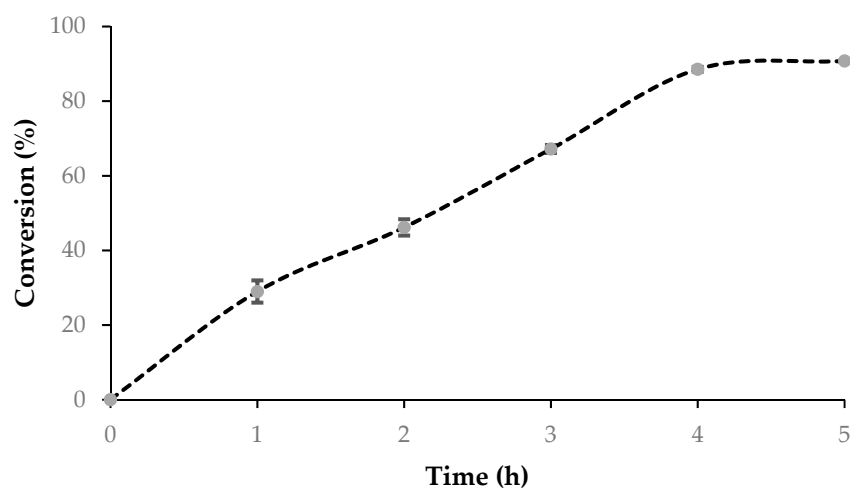
Figure 5. Esterification of oleic acid with 1-octanol under optimal conditions. Evaluation of the reaction time. Reaction conditions: 1 mmol of oleic acid, 2 mmol of 1-octanol, 1 mL n-heptane, 10% of biocatalyst based on OA mass, and 30 °C.
