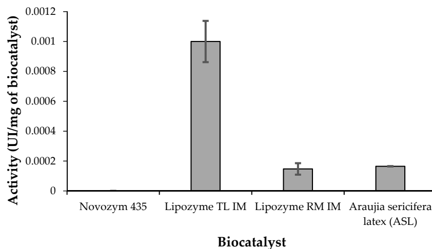
Figure 13. Hydrolysis of p -nitrophenyl palmitate using different biocatalyst (pH 8.0, 0.1 M Tris-HCl, 0.0075% ( v/v ) Triton X-100, 30 °C, 2.5 mg of biocatalyst, and 10 min).
