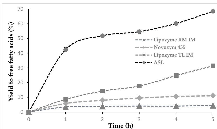
Figure 11. Hydrolysis of soybean oil using different biocatalyst. Reaction conditions: 1 mmol of soybean oil, 10 mmol of water, 1 mL n-heptane, 15% of biocatalyst based on soybean oil mass, and 30 °C. Biocatalyst: ASL, Novozym 435, Lipozyme RM IM, Lipozyme TL IM.
