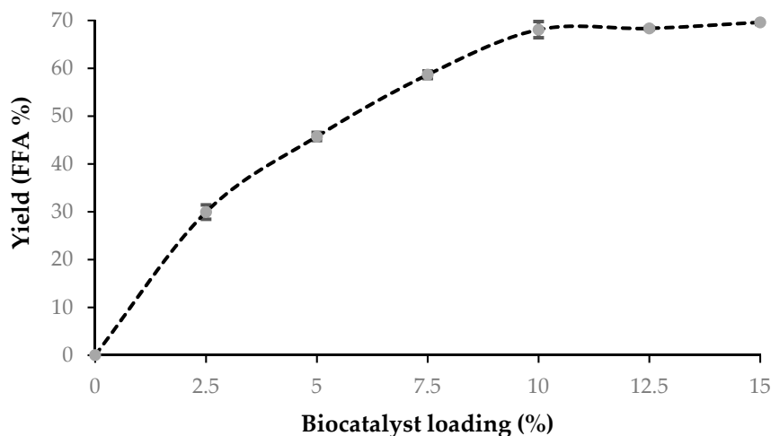
Figure 9. Hydrolysis of soybean oil using different biocatalyst loading. Reaction conditions: 1 mmol of soybean oil, 9 mmol of water, 1 mL n-heptane, 30 °C, and 5 h.
