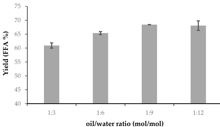
Figure 7. Hydrolysis of soybean oil using different oil/water molar ratios. Reaction conditions: 1 mmol of soybean oil, 1 mL n-heptane, 10% of biocatalyst based on soybean oil mass, 30 °C, and 5 h.
