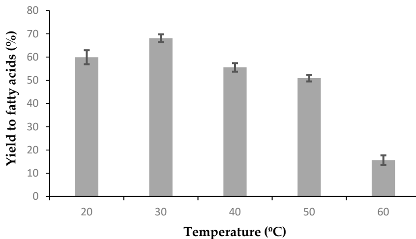
Figure 8. Hydrolysis of soybean oil at different reaction temperatures. Reaction conditions: 1 mmol of soybean oil, 9 mmol of water, 1 mL n-heptane, 5 h, and 10% of biocatalyst based on soybean oil mass.
