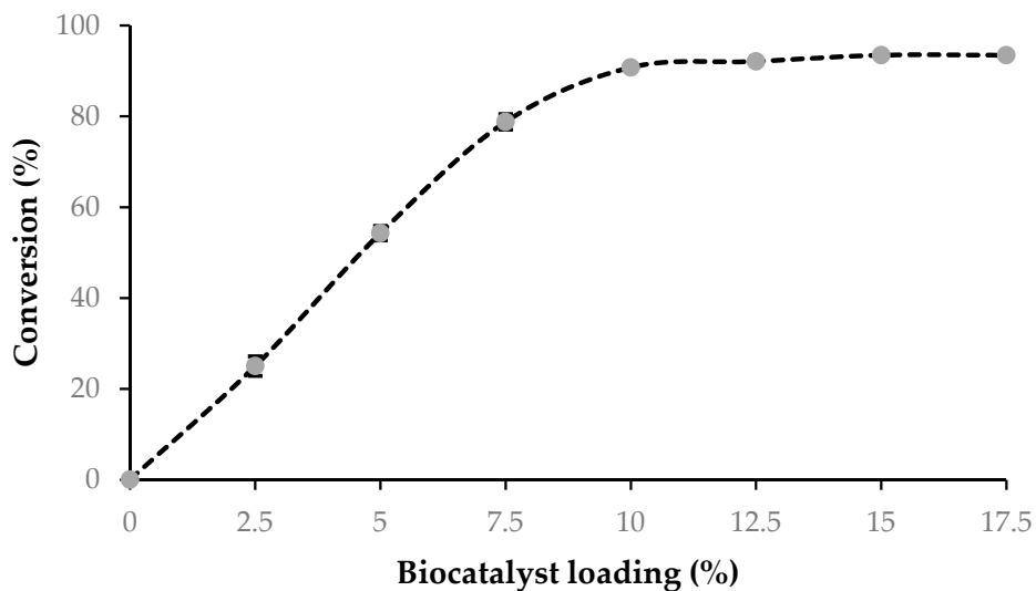
Figure 3. Esterification of OA and 1-octanol using different biocatalyst loading. Reaction conditions: 1 mmol of OA, 2mmol of 1-octanol, 1 mL n-heptane, 30 °C, and 5 h.
