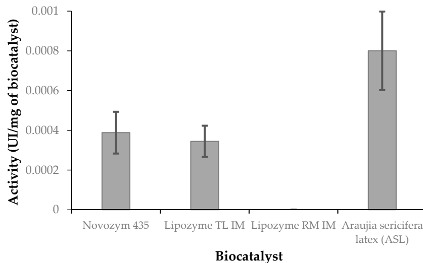
Figure 12. Hydrolysis of p -nitrophenyl laurate using different biocatalyst (pH 8.0, 0.1 M Tris-HCl, 0.0075% ( v/v ) Triton X-100, 30 °C, 5 mg of biocatalyst, and 6 min).
