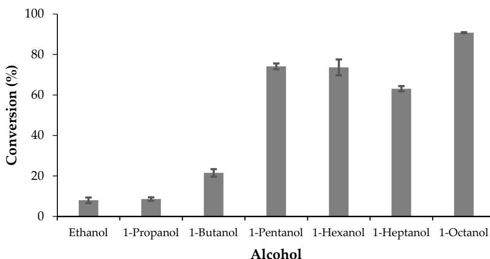
Figure 1. Esterification of OA with alcohols with different length of carbon chain. Reaction conditions: 1 mmol of OA, 2 mmol of alcohol, 1 mL n-heptane, 30 °C, 5 h, and 10% of biocatalyst based on OA mass.
