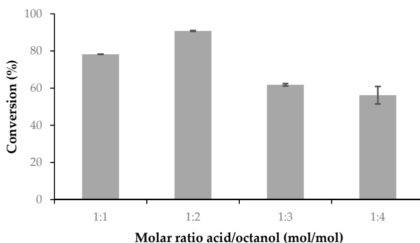
Figure 4. Esterification of OA with 1-octanol with different acid/octanol molar ratios. Reaction conditions: 1 mmol of OA, 1 mL n-heptane, 10% of biocatalyst based on OA mass, 30 °C, and 5 h.
