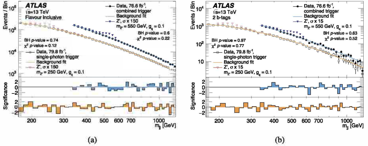
Fig. 1. Dijet mass distributions for the (a) flavour-inclusive and (b) b -tagged categories. In both figures, the distribution for the sample collected using the combined trigger with E_T^{\gamma} > 95 GeV and two p_T^{\text{jet}} > 25 GeV jets (filled circles) and the distribution for the sample collected using the single-photon trigger with E_T^{\gamma} > 150 GeV (open squares) are shown separately. The solid lines indicate the background estimated from the fitting method described in the text. Also shown are the p -values both by a \chi^2 comparison of data to background estimate and by BumpHunter (BH). The solid and empty triangles represent a Z' injected signal with g_q = 0.1 , masses of 550 and 250 GeV, respectively, where the theory-cross section is multiplied by the factor shown in the legend. The bottom panels show the significances of bin-by-bin differences between the data and the fits for the combined trigger (middle) and single-photon trigger (bottom). These Gaussian significances are calculated from the Poisson probability, considering only statistical uncertainties on the data.
