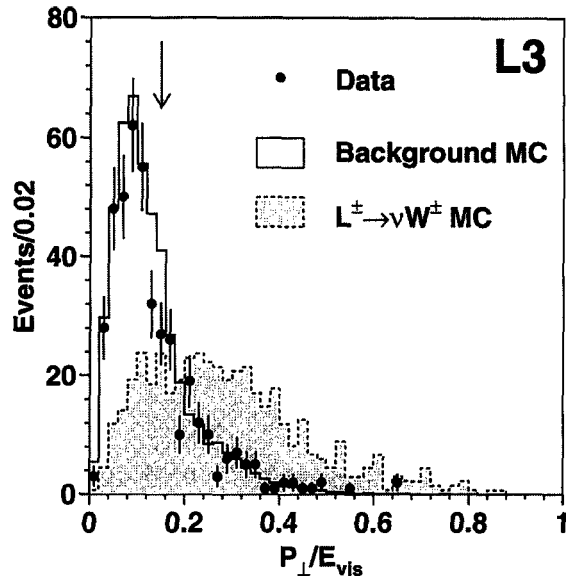
Fig. 4. The distribution of the transverse momentum, P_\perp , normalised to the total visible energy, E_{\text{vis}} . The dots are the data (taken at \sqrt{s} = 161 GeV and 172 GeV), the solid histogram is the background Monte Carlo. The dashed histogram is a predicted signal e^+e^- \rightarrow L^+L^- with m_{L^\pm} = 75 GeV. The normalization for the signal Monte Carlo is scaled by a factor of 10 for better visibility. The arrow indicates the corresponding value of the applied cut.
