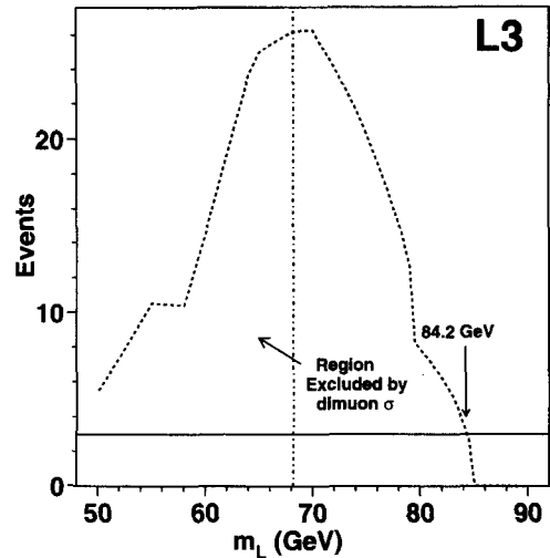
Fig. 7. The dashed line represents the expected number of stable charged heavy lepton events in the L3 data at \sqrt{s} = 133\text{--}172 GeV as a function of mass. The solid line is the 95% C.L. limit in the data. The arrow indicates the 95% C.L. lower limit obtained for stable charged heavy lepton mass. Also indicated by the dot-dashed line is the region excluded by the dimuon cross section measurement.
