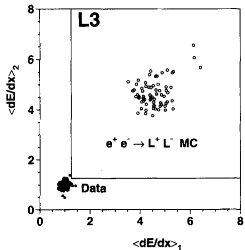
Fig. 6. The normalized measured track energy loss of track 2 vs track 1 for the data (solid circles) taken at \sqrt{s} = 172 GeV and the expected signal (arbitrary normalization) for a mass 84 GeV stable heavy charged lepton (open circles). The lines represent the corresponding value of the applied cut.
