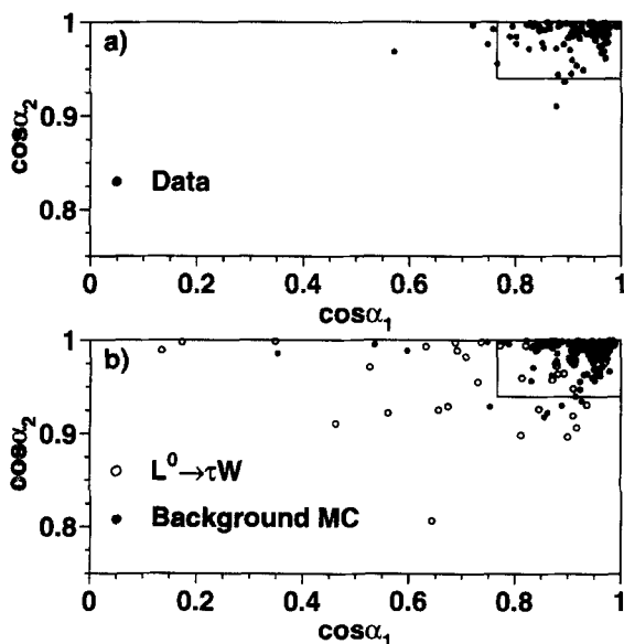
Fig. 1. a) \cos \alpha_1 vs \cos \alpha_2 , where \alpha_1 is the angle between most isolated track and the track nearest to it and \alpha_2 is the angle between the second most isolated track and the track nearest to it, for the data taken at \sqrt{s} = 161 GeV and 172 GeV. The lines represent the cut. b) \cos \alpha_1 versus \cos \alpha_2 . The black circles represent the background Monte Carlo. The open circles are the predicted signal e^+e^- \rightarrow L^0L^0 , where L^0 is of the Dirac type with m_{L^0} = 70 GeV. The normalization for the signal Monte Carlo is scaled by a factor of 2 for better visibility. The lines represent the corresponding value of the applied cut.
