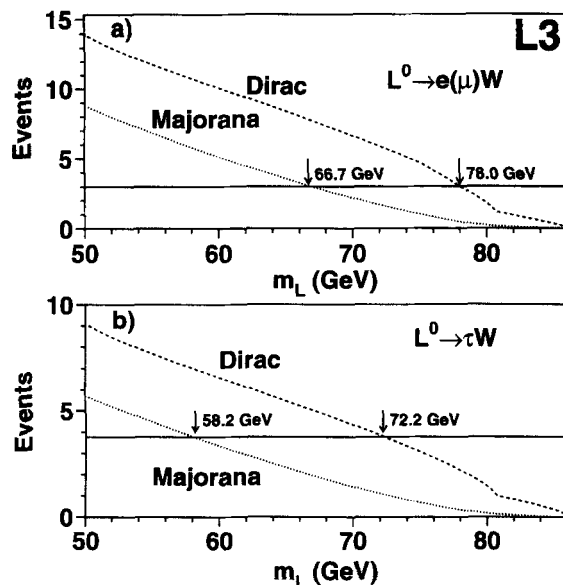
Fig. 2. a) Expected number of events (in the 161 and 172 GeV data) as a function of neutral heavy lepton mass for decays into electrons or muons. The dashed and dotted curves represent the expectations for sequential Dirac and Majorana neutrinos, respectively. The line represents the 95% C.L. limit. The arrows indicate the 95% C.L. lower limit obtained for heavy neutral lepton mass. b) Expected number of events (in the 161 and 172 GeV data) as a function of the neutral heavy lepton mass for decays into taus.
