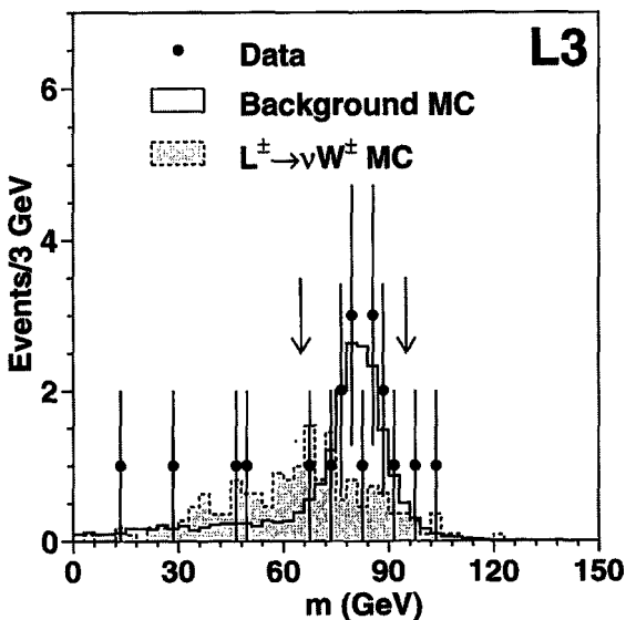
Fig. 3. The invariant mass, m , of the isolated lepton and missing momentum. The dots are the data (taken at \sqrt{s} = 161 and 172 GeV), the solid histogram is the background Monte Carlo. The dashed histogram is a predicted signal e^+e^- \rightarrow L^+L^- with m_{L^\pm} = 75 GeV. The normalization for the signal Monte Carlo is scaled by a factor of 2 for better visibility. The arrows indicate the corresponding value of the applied cut.
