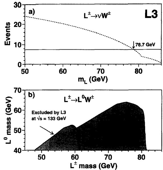
Fig. 5. a) The dashed line represents the expected number of events (in the 161 and 172 GeV data) as a function of charged heavy lepton mass for decays into light neutrino. The arrow indicates the 95% C.L. lower limit obtained for heavy charged lepton mass. b) The 95% confidence level limits on the charged heavy lepton mass m_{L^\pm} and the associated neutral heavy lepton mass m_{L^0} assuming L^0 is stable at \sqrt{s} = 172 GeV. Also shown is the limit from the previous L3 result at \sqrt{s} = 133 GeV.
