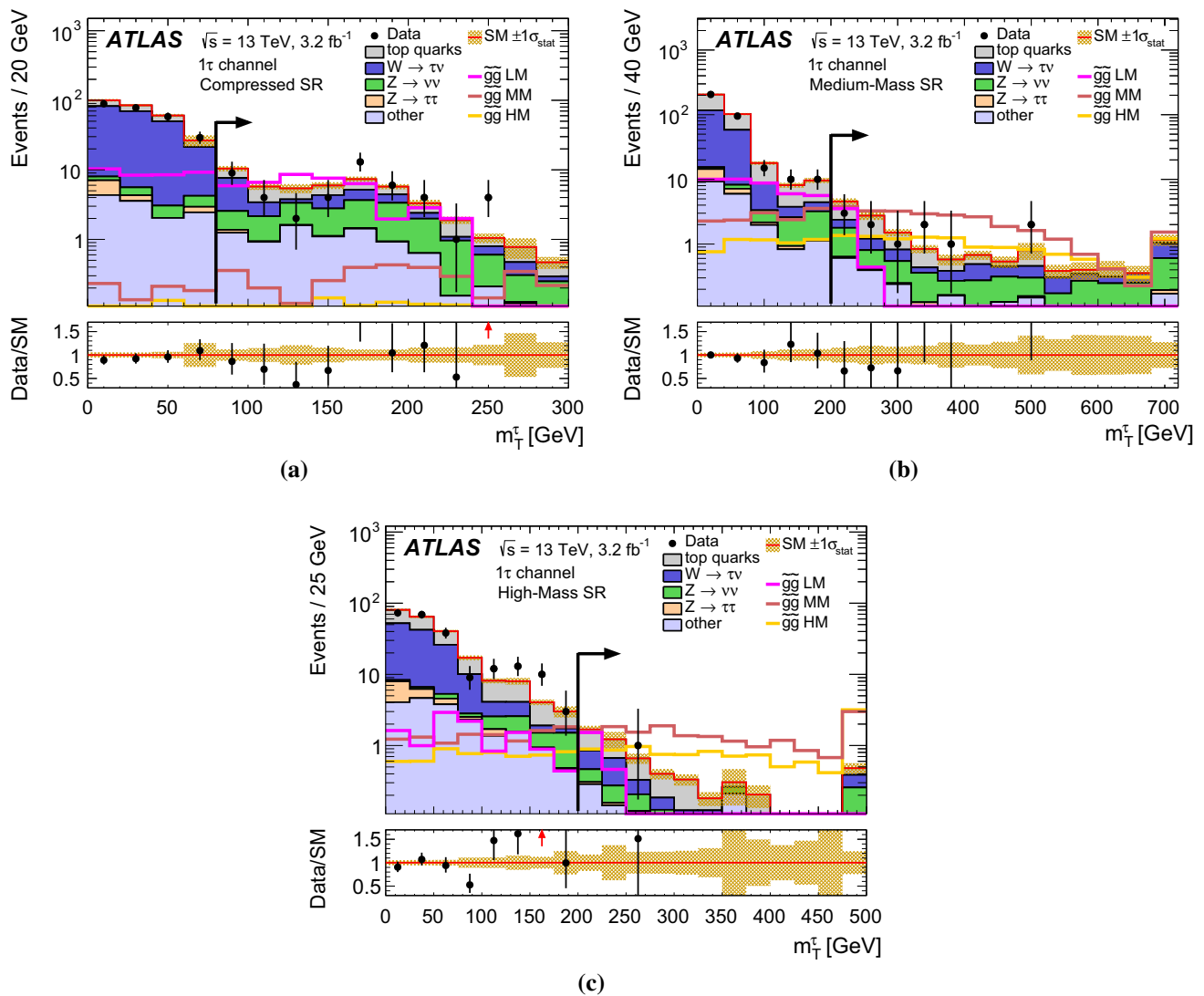
Fig. 6 m_T^\tau distributions for “extended SR selections” of the 1 \tau channel, for a the Compressed SR selection without the m_T^\tau > 80 GeV requirement, b the Medium-Mass SR selection without the m_T^\tau > 200 GeV requirement, and c the High-Mass SR selection without the m_T^\tau > 200 GeV requirement. The last bin includes overflow events. The shaded bands indicate the statistical uncertainties in the background predictions. Red arrows in the data/SM ratio indicate bins where the
