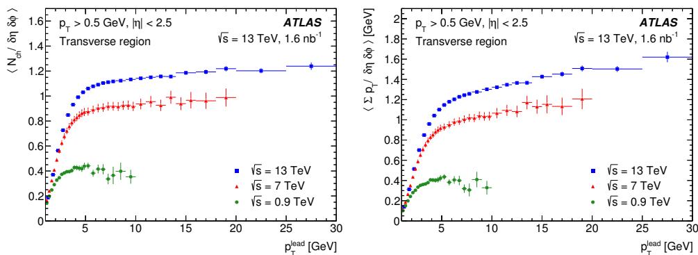
Figure 7. Mean charged-particle multiplicity (left) and \sum p_T (right) densities as a function of transverse momentum of the leading charged particle measured for \sqrt{s} = 0.9, 7 \text{ TeV} [1] and 13 TeV centre-of-mass energies. The fiducial acceptance definitions of the \sqrt{s} = 0.9 and 7 TeV measurements did not exclude charged strange baryons, but this effect is limited to a few percent at most.
