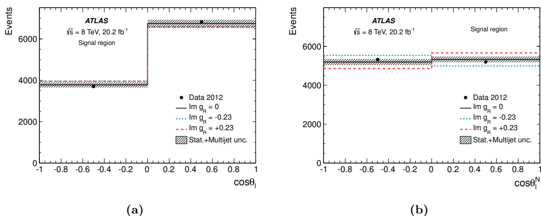
Figure 8. Comparison of the distributions observed in the signal region with the distributions predicted as a function of \text{Im } g_R for the angular observables from which the asymmetries used to set limits on this coupling are measured: (a) \cos\theta_\ell for A_{\text{FB}}^\ell and (b) \cos\theta_\ell^N for A_{\text{FB}}^N . The predicted distributions are determined by adding the signal and background contributions normalised to the results of the maximum-likelihood fit. The template signal distributions are taken from the PROTOS samples generated with \text{Im } g_R = 0 (Standard Model parameterisation) and \text{Im } g_R = \pm 0.23 . The corresponding parton-level values for the A_{\text{FB}}^N asymmetry are 0 and \pm 0.10 , respectively. For A_{\text{FB}}^\ell the predicted values are 0.45 for \text{Im } g_R = 0 and 0.34 for \text{Im } g_R = \pm 0.23 . The uncertainty bands include the statistical post-fit uncertainty, the uncertainty due to the limited size of the simulation samples and the uncertainty in the normalisation of the multijet background, added in quadrature.
