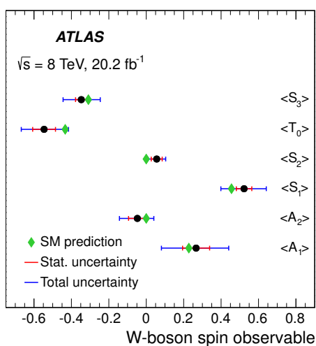
Figure 10. Summary of the measured values of the W -boson spin observables and comparison with the Standard Model predictions.
