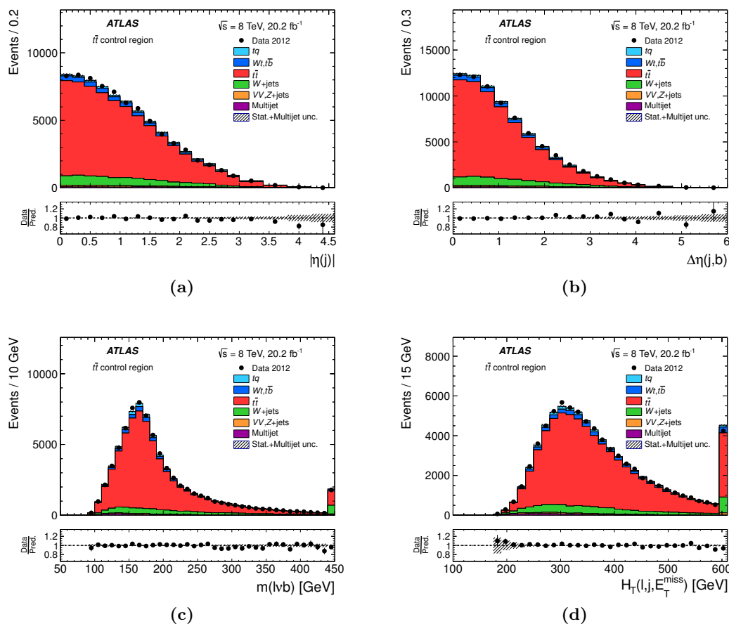
Figure 4. Distributions of the selection variables in the t\bar{t} control region: (a) |\eta| of the untagged jet, (b) separation in \eta between the untagged and b -tagged jets, (c) reconstructed top-quark mass, and (d) scalar sum of the p_T of the lepton, the p_T of the jets and E_T^{\text{miss}} . The observed distributions are compared to the predicted signal and background distributions, normalised to the results of the maximum-likelihood fit. The labels tq and t\bar{b} refer to the t -channel and s -channel single-top-quark processes, respectively, and VV to diboson production. The uncertainty bands include the statistical post-fit uncertainty, the uncertainty due to the limited size of the simulation samples and the uncertainty in the normalisation of the multijet background, added in quadrature. The last bin of the histograms includes overflows. The lower panels show the ratio of data to prediction.
