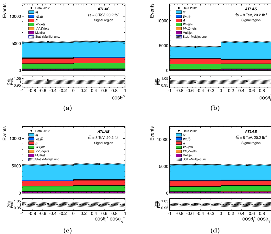
Figure 7. Distributions in the signal region of the angular observables used to measure the various asymmetries: (a) \cos \theta_\ell^N for A_{\text{FB}}^N , (b) \cos \theta_\ell^T for A_{\text{FB}}^T , (c) \cos \theta_\ell^* \cos \phi_N^* for A_{\text{FB}}^{N,\phi} , and (d) \cos \theta_\ell^* \cos \phi_T^* for A_{\text{FB}}^{T,\phi} . The observed distributions are compared to the predicted signal and background distributions, normalised to the results of the maximum-likelihood fit. The template t -channel distributions are taken from the baseline POWHEG-BOX sample. The labels tq and t\bar{b} refer to the t -channel and s -channel single-top-quark processes, respectively, and VV to diboson production. The uncertainty bands include the statistical post-fit uncertainty, the uncertainty due to the limited size of the simulation samples and the uncertainty in the normalisation of the multijet background, added in quadrature. The lower panels show the ratio of data to prediction.
