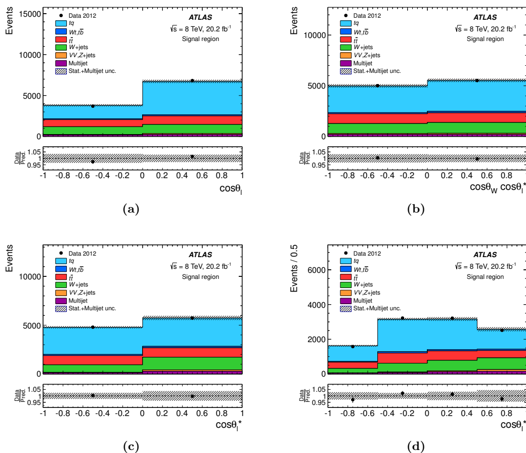
Figure 6. Distributions in the signal region of the angular observables used to measure the various asymmetries: (a) \cos \theta_\ell for A_{\text{FB}}^\ell , (b) \cos \theta_W \cos \theta_\ell^* for A_{\text{FB}}^{W\ell} , (c) \cos \theta_\ell^* with two bins for A_{\text{FB}} , and (d) \cos \theta_\ell^* with four bins for A_{\text{EC}} . The observed distributions are compared to the predicted signal and background distributions, normalised to the results of the maximum-likelihood fit. The template t -channel distributions are taken from the baseline POWHEG-BOX sample. The labels tq and t\bar{b} refer to the t -channel and s -channel single-top-quark processes, respectively, and VV to diboson production. The uncertainty bands include the statistical post-fit uncertainty, the uncertainty due to the limited size of the simulation samples and the uncertainty in the normalisation of the multijet background, added in quadrature. The lower panels show the ratio of data to prediction.
