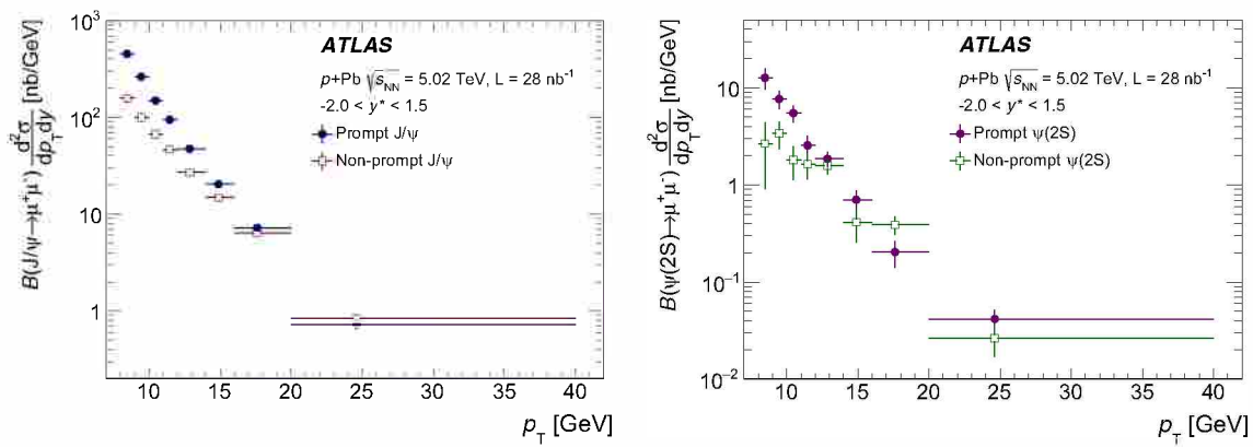
Fig. 7 The differential cross section times dimuon branching fraction of prompt and non-prompt J/\psi (left) and \psi(2S) (right) as a function of transverse momentum p_T in p+Pb collisions at \sqrt{s_{NN}} = 5.02 TeV. The horizontal position of each data point indicates the mean of the
