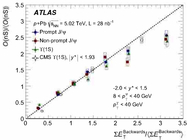
Fig. 14 Self-normalised yield for prompt J/\psi , non-prompt J/\psi and \Upsilon(1S) , compared to \Upsilon(1S) self-normalised yield ratio measured by CMS [26]. The horizontal position of each data point represents the normalised mean value of the \Sigma E_T^{\text{Backwards}} distribution in minimum-bias data sample. The error bar represents statistical uncertainties, and the vertical size of box underneath the data point represents the systematic uncertainties. The dotted line is a linear function with a slope equal to unity
