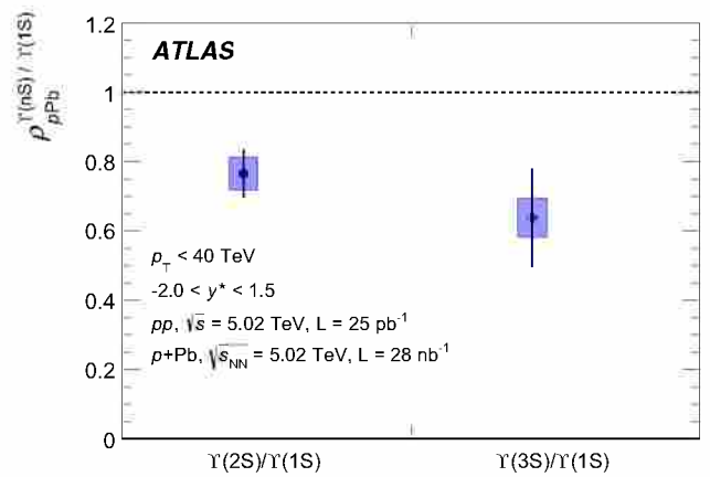
Fig. 16 The bottomonium double ratio, \rho_{pPb}^{\Upsilon(nS)/\Upsilon(1S)} , integrated in the whole measured p_T and y^* range. The vertical error bars correspond to the statistical uncertainties. The vertical sizes of boxes around the data points represent the systematic uncertainties
