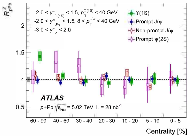
Fig. 13 Prompt and non-prompt J/\psi , prompt \psi(2S) and \Upsilon(1S) to Z boson yield ratio, R_{pPb}^Z , as a function of event centrality in p+Pb collisions. The ratio is normalised to the ratio integrated in the centrality range 0–90%. The error bars represent statistical uncertainties. The vertical sizes of coloured boxes around the data points represent the uncorrelated systematic uncertainties, and the vertical size of the left-most grey box around R_{pPb}^Z = 1 represents the correlated systematic uncertainty
