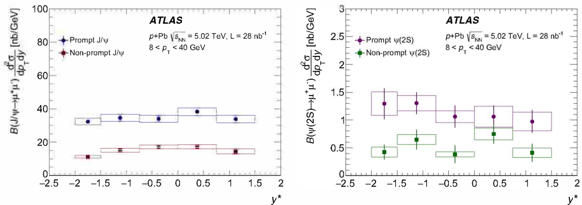
Fig. 8 The differential cross section times dimuon branching fraction of prompt and non-prompt J/\psi (left) and \psi(2S) (right) as a function of centre-of-mass rapidity y^* in p+Pb collisions at \sqrt{s_{NN}} = 5.02 TeV. The horizontal position of each data point indicates the mean of the
