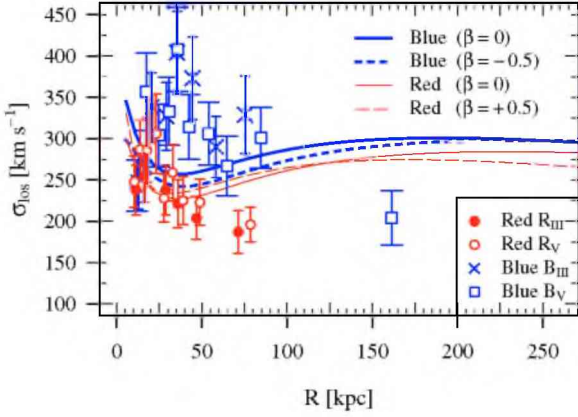
Fig. 21. Comparison to the “nested halo” mass profile by Ikebe et al. (1996) . Here, we plot the dispersion profiles expected for their Model 1, see text for details. The thick curves are the dispersion profiles for the blue GCs, where the solid and dashed lines correspond to \beta = 0 and \beta = -0.5 , respectively. The thin lines show the models for the red GCs. The solid line is \beta = 0 , and the long-dashed line shows the model for \beta = +0.5 . The data for the red GC samples RIII and RV are shown as dots and circles, respectively. The corresponding blue samples BIII and BV are shown as crosses and unfilled squares, respectively.
