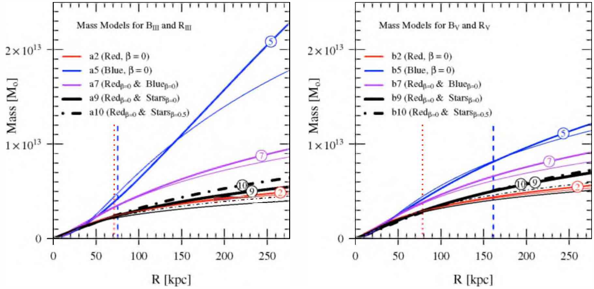
Fig. 19. Left panel: mass profiles derived for the GC dispersion profiles RIII and BIII. The thick lines with labels referring to the identifiers in Table 6 show the mass assuming an NFW-type dark halo. The cored Burkert halos are shown as thin curves with the same line style. For a given tracer population, the Burkert halo is less massive than the best-fit NFW halo. Right panel: the same for the extended data sets RV and BV (i.e. including velocities from B+07). In both panels, the dotted and dashed vertical lines indicate the radial distance of the outermost velocity dispersion data point for the red and blue GCs, respectively (cf. Table A.2).
