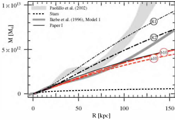
Fig. 22. Comparison to X-ray measurements. The grey area shows the range of the mass models presented by Paolillo et al. (2002) . The thick solid line shows the mass derived by Ikebe et al. (1996) (their Model 1). The thin solid line indicates the mass profile derived in Paper I. The dash-dotted curves are the two halos presented in Richtler et al. (2008) : the more massive one (labelled R1) has the parameters r_s = 50 kpc and \rho_s = 0.0085 M_\odot \text{pc}^{-3} . The halo derived for the “safe” sample in Richtler et al. (2008) (R2) has r_s = 50 kpc and \rho_s = 0.0065 M_\odot \text{pc}^{-3} . The dashed and long-dashed curves are the best-fit NFW mass profiles a10 and b10 derived in this work (cf. Table 6). The stellar mass is shown as a short-dashed line.
