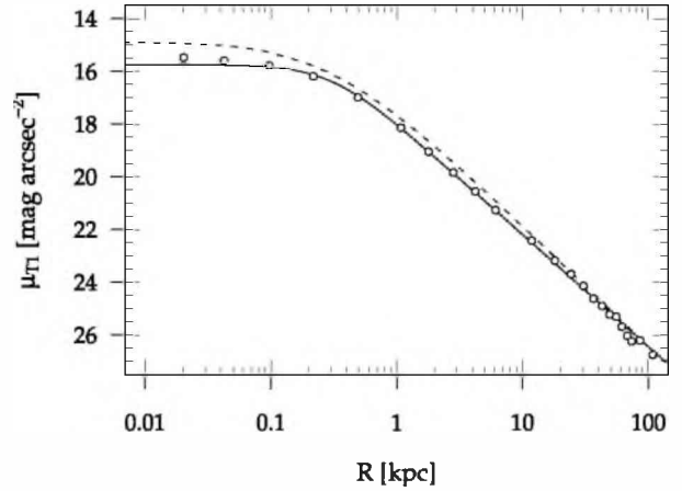
Fig. 16. Comparison between different deprojections of the surface brightness profile of NGC 1399: the dashed curve is the re-projection of the luminosity density profile as given in D+03 (Eq. (15)). The solid curve shows the fit to the data (Eq. (12)), which corresponds to the re-projection of Eq. (14).
