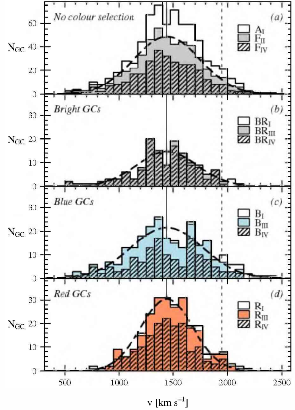
Fig. 11. Velocity histograms. a) the unfilled histogram shows all 693 GCs (AI). The solid histogram bars are the faint ( m_R > 21.1 ) GCs outside the 3' radius around NGC 1404 (i.e. sample FII), and the dashed histogram is the same for the “Class A” velocity measurements after outlier rejection (sample FIV). b) the bright ( m_R \leq 21.1 ) GCs, BRI, BRIII, and BRIV. Panels c) and d) show the same for blue and red GCs, respectively. In all panels, the solid and dashed vertical lines show the systemic velocity of NGC 1399 and NGC 1404, respectively. The dashed curve is a Gaussian with the width as given in Table 3 for the data represented as solid histogram (i.e. FII, BRIII, BIII, and RIII, respectively). Note that the range of the y -axis has been adjusted for easier comparison, with panel a) having twice the range of the subsequent plots.
