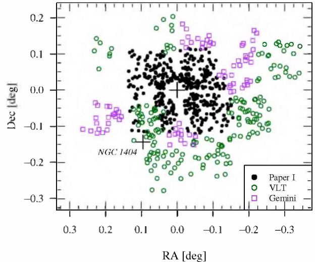
Fig. 1. Spatial distribution of spectroscopically confirmed GCs with respect to NGC 1399 (0,0). Dots represent GCs from Paper I. Circles and squares are the new GCs, measured using VLT/FORS 2 and Gemini/GMOS, respectively. North is to the top and East is to the left. The positions of NGC 1399 and NGC 1404 are marked by crosses.
