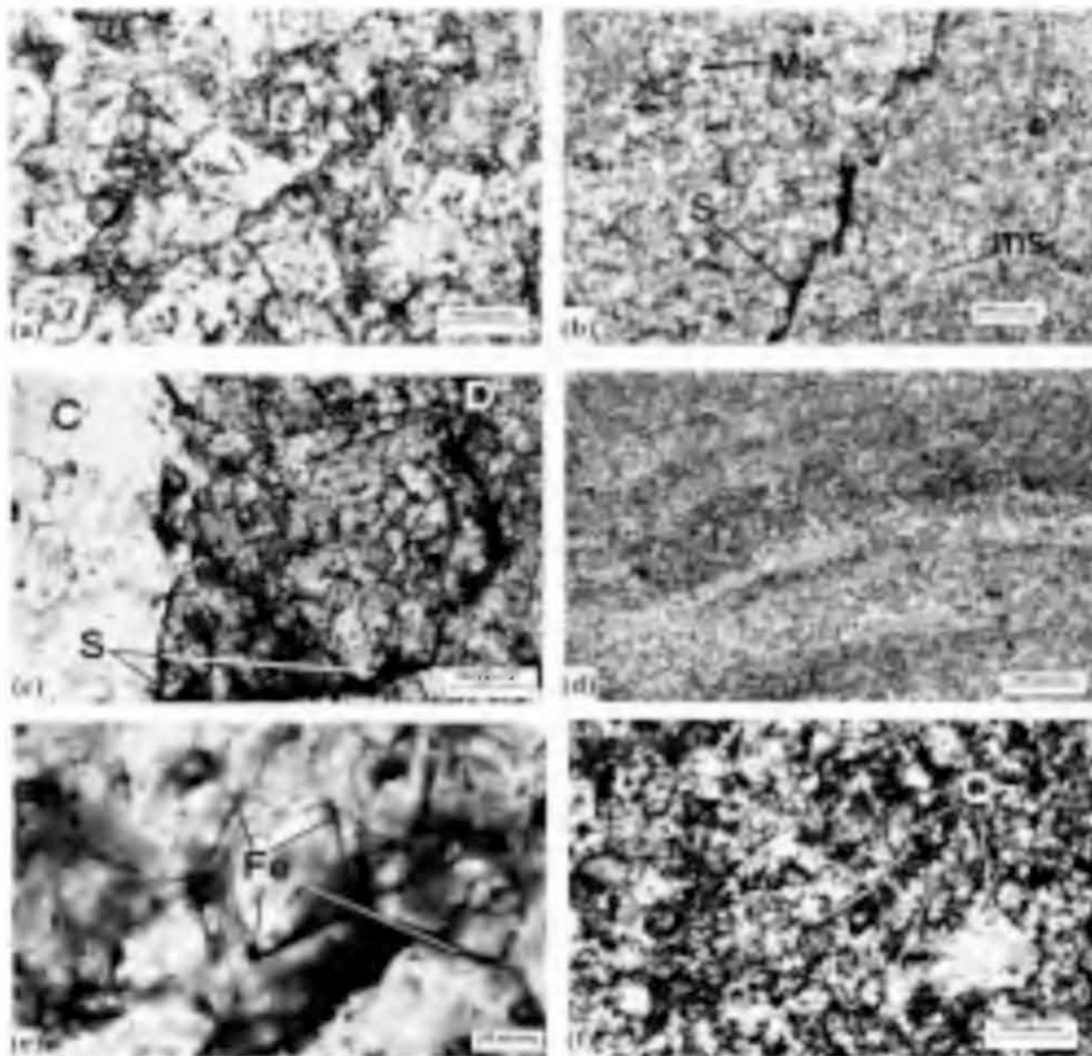
Fig 7 Thin sections of C Facies La Placeres quarry (a) Binodal dolomitized rhombohedral carbonate crystals (b) Estandia La Siempre Verde quarry Idem Ms macrosparte ms microsparte Sample stained with Alizarin-red S stylolite filled with ferric oxides (c) Staining with Alizarin-red shows that dolomitization was complete, (D dolomite, dark part of the photograph) Calcite fills fractures (C white part of the photograph) (d) Banded structure (stromatolites) (e) Epitaxial calcite (C) on dolomite crystals (arrow) Fe ferric oxides Sample stained with Alizarin-red (f) La Placeres quarry Quartz pseudomorphous after dolomite rhombohedral crystals Quartz Qz (X nicols)
