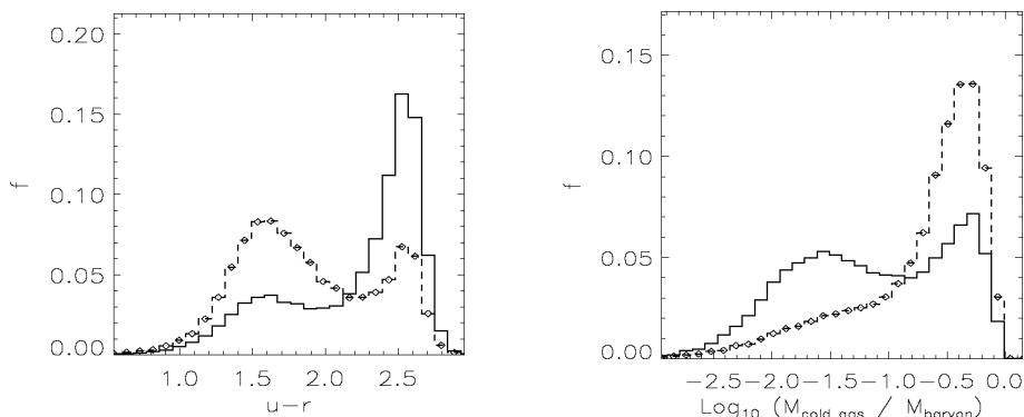
Figure 1. The (u - r) colour distributions (left-hand panel) and cold gas fraction distributions (right-hand panel) for both galaxies in pairs (solid line) and in the Control 1 (dashed line). Error bars are standard deviations computed for 100 realizations of CS (see the text for more details).
