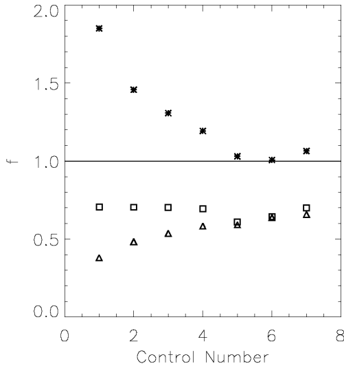
Figure 7. Control efficiency C_e (asterisk) and red fractions ( u - r > 2 ; open triangles) of all analysed CS, defined with numbers from 1 to 7 (Table 1). Red galaxy fractions computed for each corresponding galaxy pair samples are also shown (open squares). The horizontal line corresponds to have no excess of red galaxy pairs with respect to the CS.
