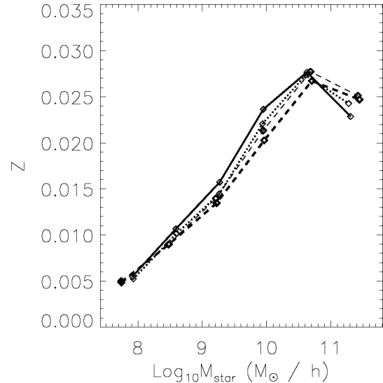
Figure 8. MZR for galaxy pairs (solid line), Control 2 (dashed thick line), Control 3 (dashed thin line) and Control 5 (dotted line).
