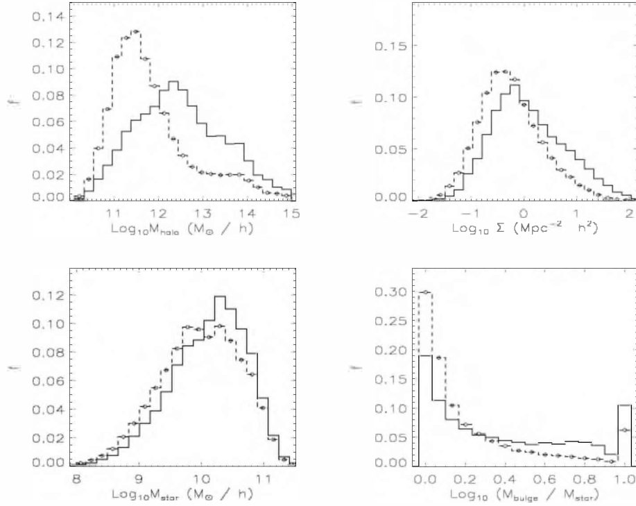
Figure 2. Histograms of the dark matter halo masses (upper-left panel), local density parameter ( \Sigma ) distributions (upper-right panel), stellar mass distributions (lower-left panel) and morphological distributions, represented by the B/T stellar masses parameter (lower-right panel), for galaxies in pairs (solid line) and in the Control 1 (dashed line).
