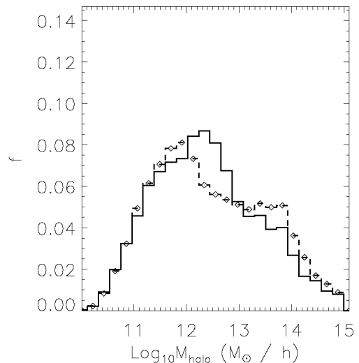
Figure 6. Dark matter halo distributions for galaxies in the Pair Catalogue (solid lines) and in Control 6 (dashed lines).
