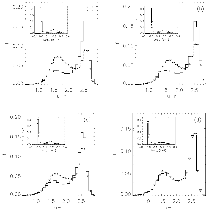
Figure 5. The u - r colour distributions for both galaxies in pairs (solid line) and without a close companion (dashed line) in Control 2 (a), Control 3 (b), Control 4 (c) and Control 5 (d). The insets show the corresponding stellar birthrate distributions, b , for both galaxies in pairs and in CS using the same convention of lines.
