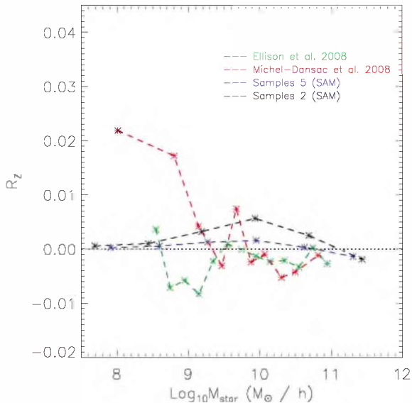
Figure 9. The pair metallicity excess, R_Z , defined as the difference between pair and CS metallicities normalized by the pair value, as a function of stellar masses. Red and green lines represent the SDSS DR4 values computed with O/H abundances kindly provided by MD08 and E08, respectively. Analogously, mock R_Z values for Samples 2 and 5 are represented by black and blue lines, respectively.
