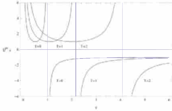
Figure 2. Mandel parameter Q_W^{sc} evaluated semiclassically by recourse to escort distributions of order q at different temperatures T (given in \hbar\omega -units).
