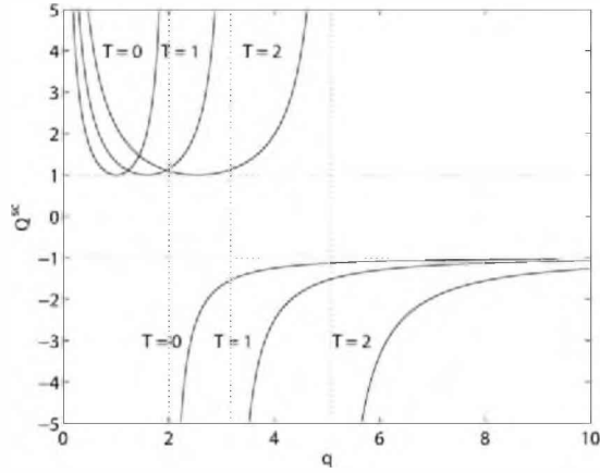
Figure 1. Mandel parameter Q^{\text{sc}} evaluated semiclassically by recourse to escort distributions of order q at different temperatures T (given in \hbar\omega -units).
