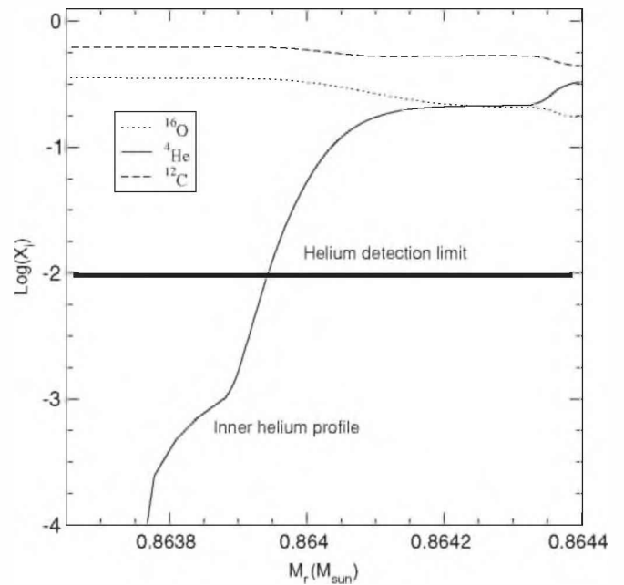
Figure 2. Internal abundance distribution of ^4\text{He} , ^{12}\text{C} , and ^{16}\text{O} for a selected model of our post-born-again 0.87 M_{\odot} sequence. The mass coordinate ranges from 0.86365 to 0.8644 M_{\odot} . Note that a non-negligible mass of residual He, of about \sim 2 \times 10^{-7} M_{\odot} , is expected below the layer having a He abundance of 0.01, the He detection limit in H1504+65 (thick line).
