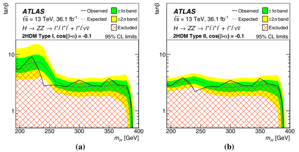
Fig. 9 The exclusion contour in the 2HDM a Type-I and b Type-II models for \cos(\beta - \alpha) = -0.1 , shown as a function of the heavy scalar mass m_H and the parameter \tan \beta . The green and yellow bands represent the \pm 1\sigma and \pm 2\sigma uncertainties in the expected limits. The hatched area shows the observed exclusion
