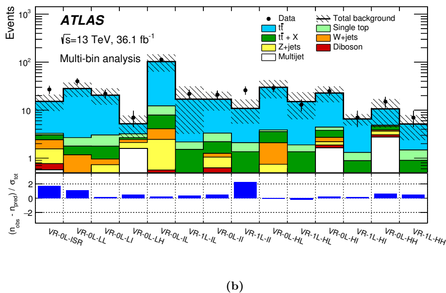
Figure 8. Results of the background-only fit extrapolated to the VRs of (a) the cut-and-count and (b) the multi-bin analyses. The t\bar{t} normalisation is obtained from the fit to the CRs shown in figure 7. The upper panel shows the observed number of events and the predicted background yield. All uncertainties defined in section 7 are included in the uncertainty band. The background category t\bar{t} + X includes t\bar{t}W/Z , t\bar{t}H and t\bar{t}t\bar{t} events. The lower panel shows the pulls in each VR.
