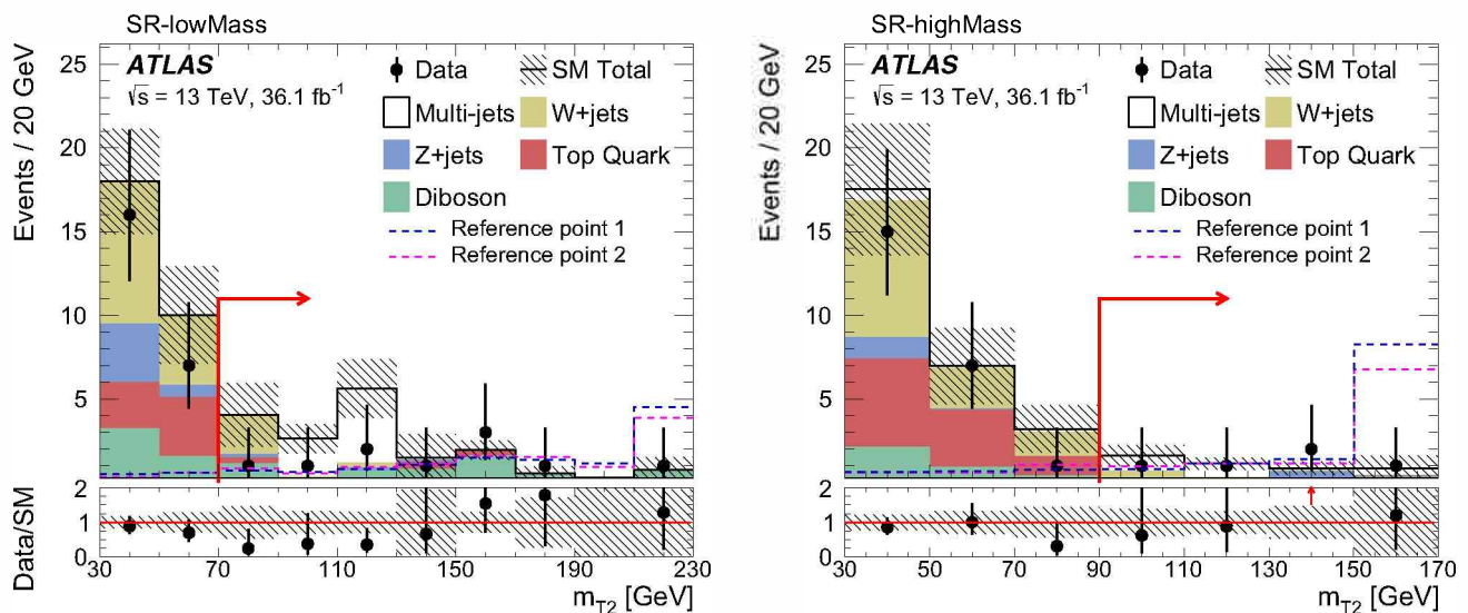
Fig. 6 The m_{T2} distribution before the m_{T2} requirement is applied for SR-lowMass (left) and SR-highMass (right) regions, where the arrow indicates the position of the cut in the signal region. The stacked histograms show the expected SM backgrounds. The multi-jet contribution is estimated from data using the ABCD method. The contributions of multi-jet and W + j ets events are scaled with the corresponding nor-
