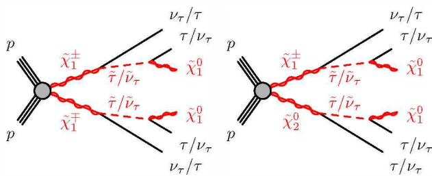
Fig. 1 Representative diagrams for the electroweak production and decay processes of supersymmetric particles considered in this work: (left) \tilde{\chi}_1^+ \tilde{\chi}_1^- and (right) \tilde{\chi}_1^\pm \tilde{\chi}_2^0 production
