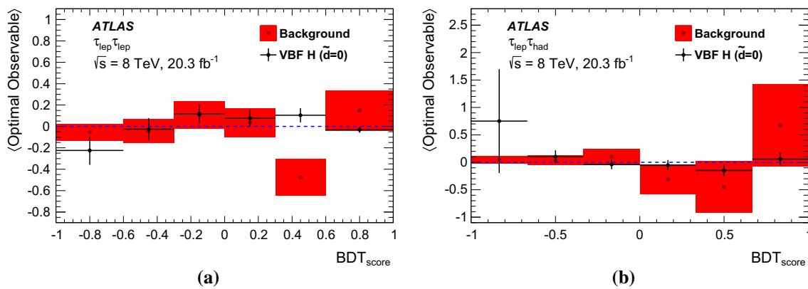
Fig. 2 Mean of the Optimal Observable as a function of the BDT_{\text{score}} for the SM signal ( black dots with error bars ) and for the sum of all background processes ( filled red area ), for the a \tau_{\text{lep}}\tau_{\text{lep}}
