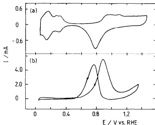
Fig. 1. Voltammograms of an electrodispersed Pt electrode ( RF=18 ) at 25^{\circ}\text{C} . (a) 1\text{ M HClO}_4 , \nu=100\text{ mV s}^{-1} ; (b) 0.5\text{ M HClO}_4+0.1\text{ M CH}_3\text{OH} , \nu=50\text{ mV s}^{-1} .
