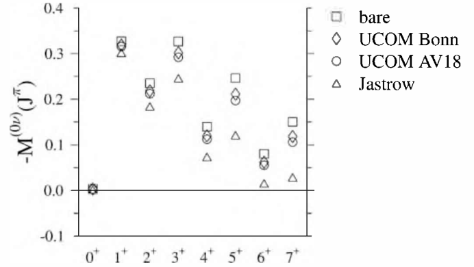
Fig. 1. Multipole decomposition of the total 0\nu\beta\beta decay matrix element M_{\text{GT}}^{(0\nu)} - (g_{\text{V}}/g_{\text{A}})^2 M_{\text{F}}^{(0\nu)} for ^{48}\text{Ca} . The cases are: no short-range correlations included (bare), with Jastrow correlations and with UCOM correlations using the Bonn-A and Argonne V18 parametrizations.
