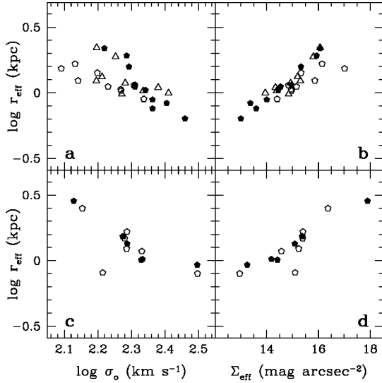
Fig. 6. \log(r_{\text{eff}}) as a function of \log(\sigma_0) a , c and \Sigma_{\text{eff}} b , d . Figures a , b show the relations for the objects that experience double starburst events; meanwhile, figures c , d correspond to the systems that present single starburst events. In all cases, open pentagons correspond to z_A , open triangles to z_C , and filled pentagons to z_D .
