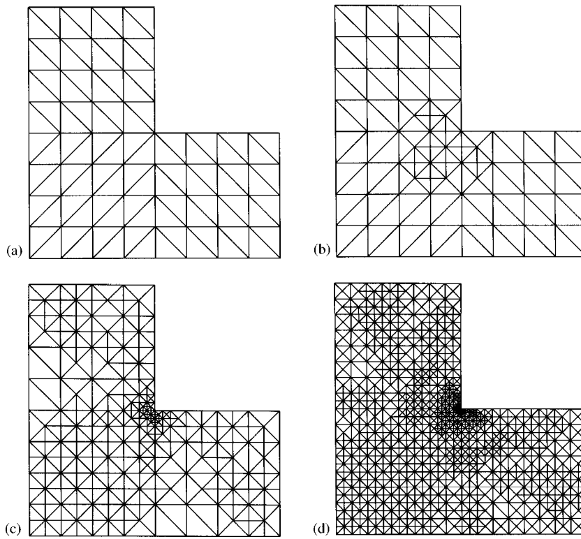
Fig. 3. Initial triangulation and some refined triangulations for Eigenmode F_1 : (a) initial triangulation; (b) first refinement step; (c) third refinement step; (d) sixth refinement step.
