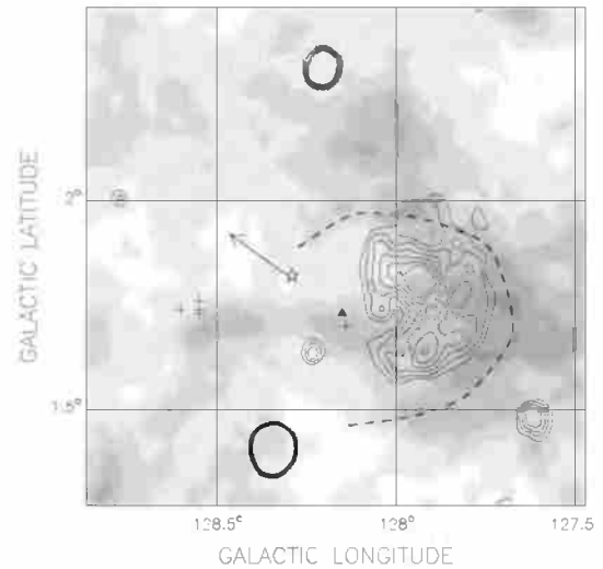
Figure 8. Radio-continuum contour at 2695 MHz superposed on the average H I distribution in the velocity interval -27.0 to -30.3 \text{ km s}^{-1} . Contour levels are at 0.1 – 0.2 \text{ K} in steps of 0.02 \text{ K} . Grey-scale steps occur from -4 to 28 in steps of 4 \text{ K} . The star symbol indicates the position of HD 10125 and the arrow the direction of its proper motion. The length of the arrow is in arbitrary units. The dashed line delineates the arc-like structure and the filled triangle shows the cavity centre position. The plus signs indicate the position of the B stars.
