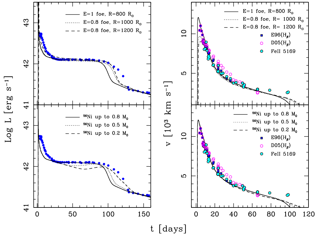
Figure 16. Comparison between models (lines) and observations (points) of SN 1999em for a low value of the pre-SN mass of M = 14 M_{\odot} and the same mass of 56 Ni as for the reference model M19R8E1.25Ni56. Left panels: bolometric LCs. Right panels: photospheric velocity evolution. Upper panels: models M14R8E1Ni56, M14R10E08Ni56, and M14R12E08Ni56 (see Table 3). Lower panels: models with different mixing of 56 Ni, E = 1 foe, and R = 800 R_{\odot} . Note that the degree of 56 Ni is indicated in each panel as a fraction of the initial mass of the model.
