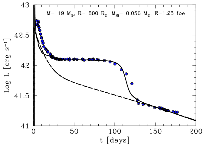
Figure 5. Bolometric LC for model M19R8E1.25Ni56 (solid line) compared with the data of SN 1999em as calculated by Bersten & Hamuy (2009; blue dots). The luminosity due to the ^{56}\text{Ni} \rightarrow ^{56}\text{Co} \rightarrow ^{56}\text{Fe} decay is also shown (dashed line). The physical parameters used in the model are indicated.
