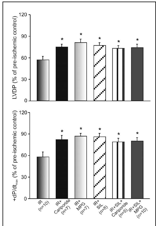
Fig. 2. Left ventricular developed pressure (LVDP) and maximal rise velocity of LVP (+dP/dt max ) at the end of the reperfusion period (expressed as a percentage of preischemic values) in all experimental groups. All interventions improved postischemic myocardial systolic function to a similar extent compared to non treated I/R. * P < 0.05 vs. I/R.
