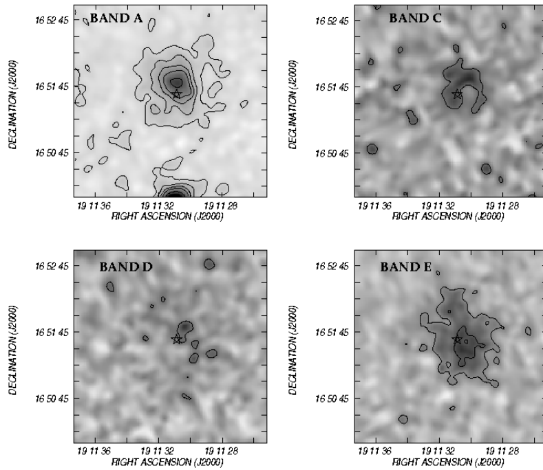
Fig. 4. MSX images towards WR 124 (star symbol). The lowest contour level represents a noise level of 4.5\sigma for band A and 3\sigma for the other bands. Low intensity regions are indicated by light greys. Top left panel: 8.28 \mu\text{m} (band A) emission. The grey scale range is -2 to 35 \text{ MJy sr}^{-1} . The contour lines are 6, 10, 14, 18, 26, 34, 42 and 50 \text{ MJy sr}^{-1} . Top right panel: band C image ( 12.1 \mu\text{m} ). The grey scale spans -75 to 130 \text{ MJy sr}^{-1} . The contour line is 57.7 \text{ MJy sr}^{-1} . Bottom left panel: band D image at 14.65 \mu\text{m} . The grey scale range is -47 to 80 \text{ MJy sr}^{-1} . The contour line is 33.6 \text{ MJy sr}^{-1} . Bottom right panel: band E image at 21.3 \mu\text{m} . The grey scale covers the range -130 to 260 \text{ MJy sr}^{-1} , contour lines are 79.5 and 159.0 \text{ MJy sr}^{-1} .
