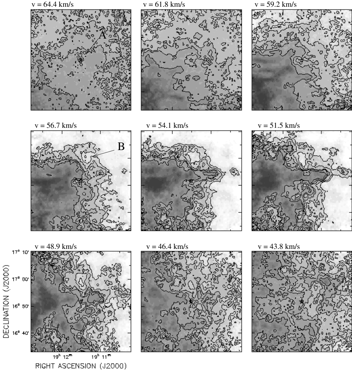
Fig. 1. Grey-scale images showing the HI gas distribution in the velocity range 64.4 to 43.8 km s -1 observed with the VLA and the 100 m Effelsberg telescope. The position of WR 124 is indicated by a star symbol. Velocity resolution is 2.6 km s -1 and the spatial resolution is 46'.5 × 45'.5 with a PA of 16'.6. The LSR velocity of each image is indicated in the top left corner. Letters A and B indicate the cavities described in the text. Contour levels with respect to the average over each image are -13, -8, -3, 0 and 5 K. Noise is 0.3 K or 1.05 mJy beam -1 .
