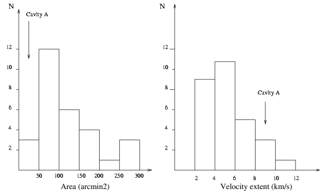
Fig. 5. Histograms of the random HI holes area and velocity extent identified in a region near the stellar position. The arrows indicate the area and velocity extent observed for cavity A.
