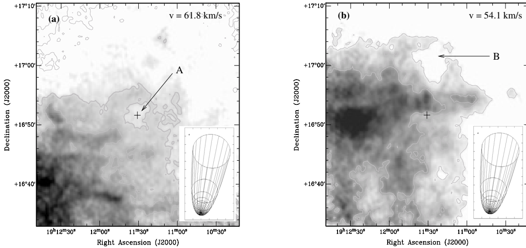
Fig. 7. a) HI emission distribution at v = 61.8 , where cavity A is best delineated. b) HI emission distribution at v = 54.1 km s -1 , where cavity B is best delineated. In both panels contour levels are -10 , 0 and 5 K. The cross marks the position of WR 124. The 3D bow shock structure for i = 30^\circ and \phi = 170^\circ is shown in the bottom right corner.
