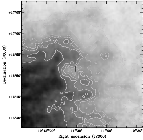
Fig. 2. Average HI brightness temperature within the LSR velocity interval 54.1 to 61.8 \text{km s}^{-1} . Contour levels with respect to the average over the image ( 28 K) are -10 , -6 , -2 , 0 , 2 and 6 K. The cross indicates the position of WR 124.
