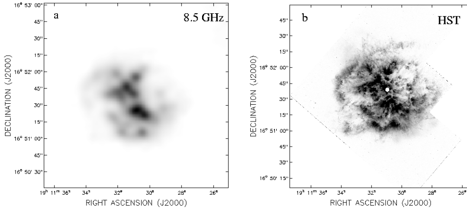
Fig. 3. a) Radio continuum image of M1-67 at 8.5 GHz with a resolution of \sim 8'' . The grey scale goes from 0 to 7 mJy beam ^{-1} (dark grey). b) HST-WFPC2 H \alpha image of M1-67 obtained by Grosdidier et al. (2001). Resolution is \sim 0''.2 .
