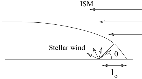
Fig. 6. Schematic side view representation of the geometry of the bow shock model. The horizontal axis represents the symmetry axis of the bow shock and l_0 is the stand-off distance.
