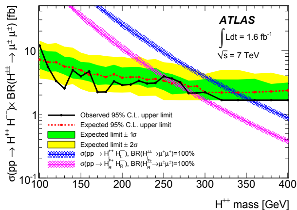
FIG. 2. Upper limit at 95% C.L. on the cross section times branching ratio for pair production of doubly charged Higgs bosons decaying to two muons. Superimposed is the predicted cross section for H_L^{++}H_L^{--} and H_R^{++}H_R^{--} production assuming a branching ratio to muons of 100%. The bands on the predicted cross sections corresponds to the theoretical uncertainty of 10%.
