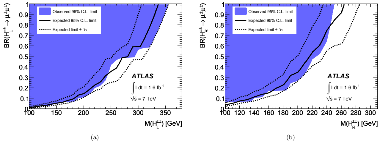
FIG. 3. Exclusion region at 95% C.L. of the H^{\pm\pm} mass as a function of the branching ratio to muon pairs, BR(H^{\pm\pm} \rightarrow \mu^{\pm}\mu^{\pm}) , for a) H_L^{\pm\pm} bosons and b) H_R^{\pm\pm} bosons. The shaded areas show the observed exclusion region, the solid lines show the expected exclusion region, and the dashed lines show the \pm 1\sigma variations of the expected exclusion region.
