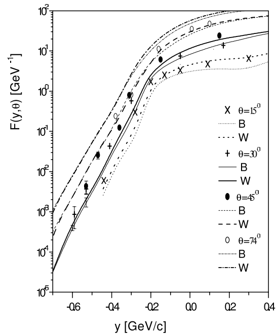
Figure 4. The scaling function F(y, \theta) for ^{56}\text{Fe} as a function of the scaling variable y for scattering angles \theta = 15^\circ, 30^\circ, 45^\circ and 74^\circ . The experimental data are from CEBAF and are indicated by points, while the results corresponding to the fits of Bodek (B) and Whitlow (W) are given by thin and thick lines, respectively. A rearrangement of data is necessary since the scaling variable and the nucleon elastic cross sections in our model are different from those adopted in the CEBAF experiment.
