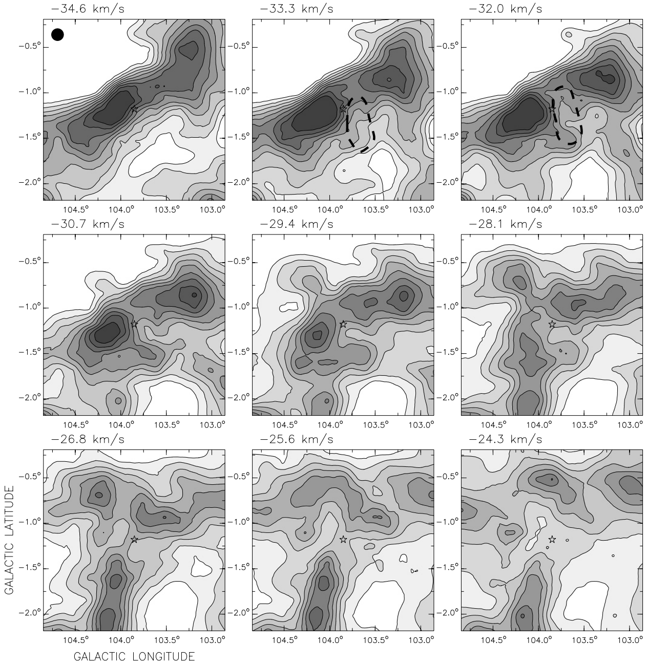
Fig. 3. WR 154 Effelsberg grey-scale images showing the HI distribution in the velocity range -34.6 to -24.3 km s ^{-1} . The half beam width (HPBW \sim 9' ) is shown in the upper left corner of the first image. The stellar position is indicated by a star symbol. The central velocity of every map is specified in the upper left corner. Contour levels are at -10 to 30 K in steps of 5 K.
