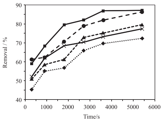
Figure 7. Methylene blue removal over the catalysts as a function of time during the Fenton reaction: AC sample (x) (activated carbon), and 2.5IAC (◆), 5IAC (▲), 10IAC (●) and 15IAC (■) samples (activated carbon-supported iron oxide). The numbers represent the iron amount (wt.%) in the solids.
