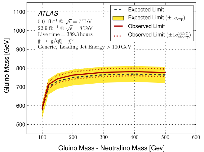
FIG. 11 (color online). Total reconstruction efficiency and Bayesian lower limits on gluino mass, as a function of the mass splitting between the gluino and the neutralino, in the generic R -hadron model with gluino lifetimes in the plateau acceptance region between 10^{-5} and 10^3 s. A 600 GeV gluino is used as a reference for the reconstruction efficiencies.
