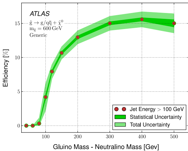
FIG. 11 (color online). Total reconstruction efficiency and Bayesian lower limits on gluino mass, as a function of the mass splitting between the gluino and the neutralino, in the generic R -hadron model with gluino lifetimes in the plateau acceptance region between 10^{-5} and 10^3 s. A 600 GeV gluino is used as a reference for the reconstruction efficiencies.
