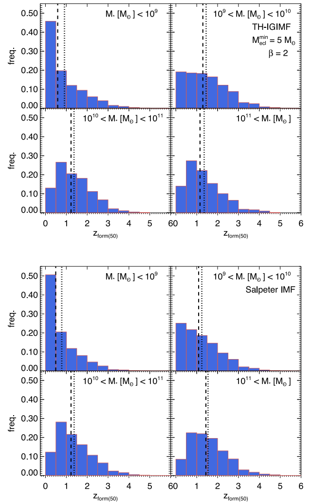
Figure 13. Distribution of formation redshifts, z_{\text{form}(50)} , for galaxies of different stellar mass, as indicated in the key for models SAGTH5B2 (top panel) and SAGS (bottom panel). The dotted and dashed lines represent the mean and median values of the distributions, respectively.
