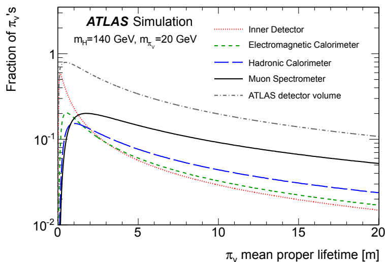
Figure 1. The probability of a \pi_\nu to decay in the ID (beyond the second layer of the pixel detector), ECal, HCal, MS and the whole ATLAS detector as a function of the \pi_\nu mean proper lifetime ( c\tau ) for |\eta| < 2.5 . The sample with m_H = 140 GeV and m_{\pi_\nu} = 20 GeV is used.
