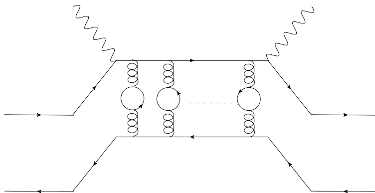
Figure 8. Forward Compton scattering at strong coupling. The meson is struck by the virtual photon indicated with a wavy line. This is the quark-model diagram which corresponds to sub-leading supergravity dual calculations of the type given by the n -flavor loop Witten's diagram. These are planar diagrams.
