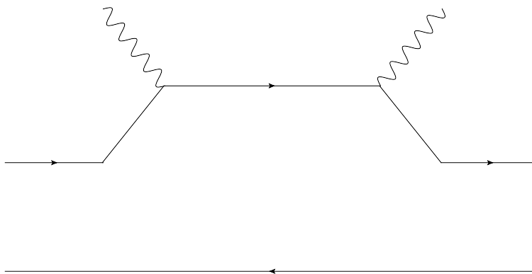
Figure 5. Forward Compton scattering from a meson in the parton model. A parton is struck by the virtual photon indicated with a wavy line.
