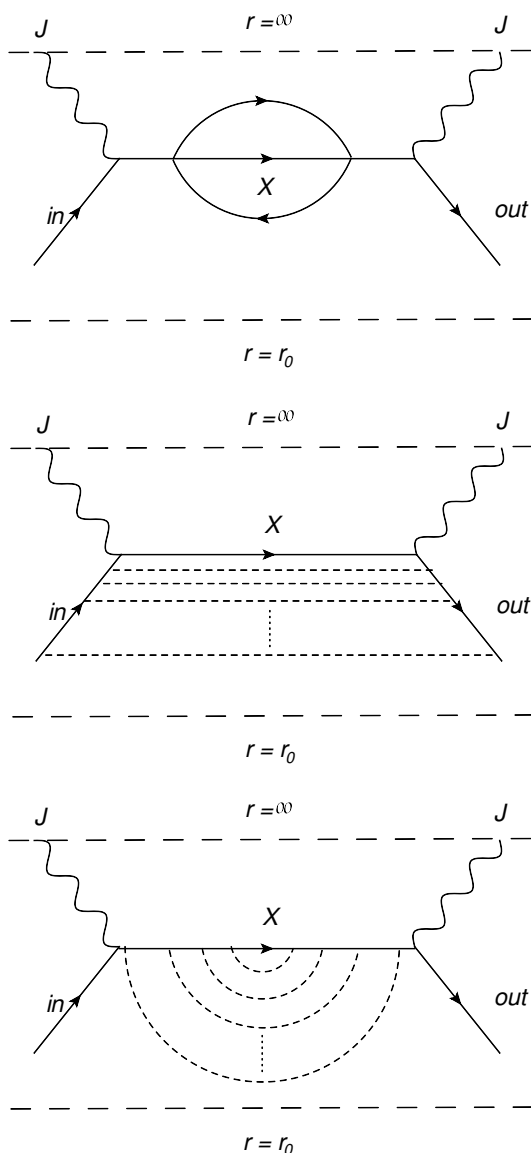
Figure 4. Illustration of some multi-loop Witten’s diagrams. Multi-loop contributions from Witten’s diagrams corresponding to sub-leading corrections to the forward Compton scattering Feynman’s diagrams contributing to DIS in four-dimensions.
