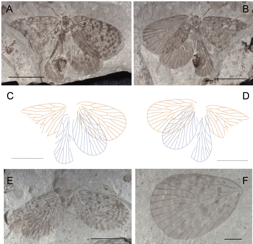
Figure 5. Photographs and line drawings of Paristopsyche angelineae gen. et sp. n. A Photograph of part of holotype, no. CNU-MEC-NN2011076p B Photograph of counterpart of holotype, no. CNU-MEC-NN2011076c C Line drawing of part of holotype, no. CNU-MEC-NN2011076p D Line drawing of counterpart of holotype, no. CNU-MEC-NN2011076c E Photograph of paratype, no. CNU-MEC-NN2009319 F Photograph of paratype, no. CNU-MEC-NN2011074. Scale bars of A–E represent 5 mm. Scale bar of F represents 1 mm.
