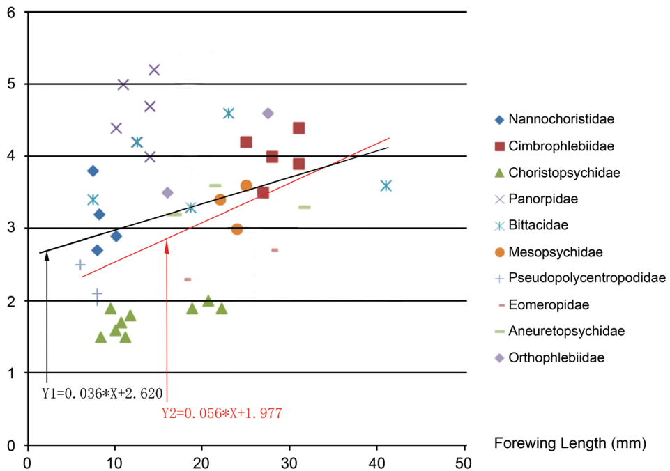
Figure 7. The ratio of forewing length (L)/width (W) vs. forewing length (in mm) of ten representative Families of Mecoptera. For all data points, the linear regression trend line is represented by Y1 = 0.036 * X + 2.620 . Excluding the data of Panorpidae, the linear regression trend line is Y2 = 0.056 * X + 1.977 .
