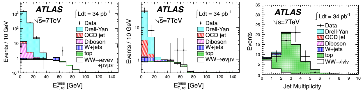
FIG. 1 (color online). E_{T,rel}^{miss} distributions for the selected ee and \mu\mu (left) and e\mu (center) events and the multiplicity distribution for jets with p_T > 20 GeV and |\eta| < 3.0 for all three dilepton channels combined (right). The distributions show events with all selection criteria applied except for E_{T,rel}^{miss} in the E_{T,rel}^{miss} distribution and the jet-veto in the jet multiplicity distribution. Simulation is used for the QCD jet and W + jets background contributions in these plots as opposed to the data-driven method used for W + jets in the signal region described in the text. The QCD jet contribution is negligible in the signal region.
