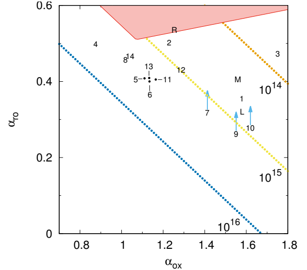
Fig. 2. Analysed sources in the spectral indices \alpha_{\text{ox}} - \alpha_{\text{ro}} plane. Lower limits are indicated with an arrow. Numbers refer to the values presented in Table 1, while letters L, M, and R refer to the objects in Landi et al. (2015b,a) associated by Landoni et al. (2015), Massaro et al. (2015b), and Ricci et al. (2015), respectively. Sources 5, 6, 11 and 13 are shown as points for the sake of clarity. The red shaded area indicates the region where the relationship describing synchrotron peak values changes its functional form, as explained in Abdo et al. (2010).
