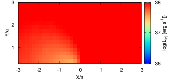
Fig. A.31. Injection luminosity of relativistic particles in the emitter in the case of fast non-radiative losses and a strong magnetic field. The normalization was set to reproduce an energy flux in the 1–30 MeV range equal to 2.6 \times 10^{-9} erg cm -2 s -1 .
