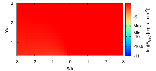
Fig. 18. As in Fig. 15 but showing the integrated energy flux in the 0.1–10 GeV energy band.
