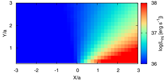
Fig. A.6. Injection luminosity of relativistic particles in the emitter in the case of slow non-radiative losses and a weak magnetic field. The normalization was set to reproduce an energy flux in the 0.1–10 GeV range equal to 2.8 \times 10^{-10} \text{ erg cm}^{-2} \text{ s}^{-1} .
