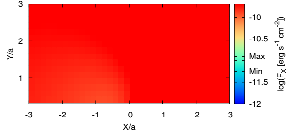
Fig. A.23. As in Fig. A.21 but showing the integrated energy flux in the 0.3–10 keV energy band.
