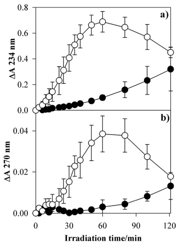
Fig. 4. Time evolution of the absorbance of (a) conjugated dienes (A234) and (b) conjugated trienes (A270) for liposomes in the presence (○) and in the absence (●) of Ptr (60 \mu\text{M} ) as a function of the irradiation time. Error bars correspond to SD from 2 to 3 different experiments.
