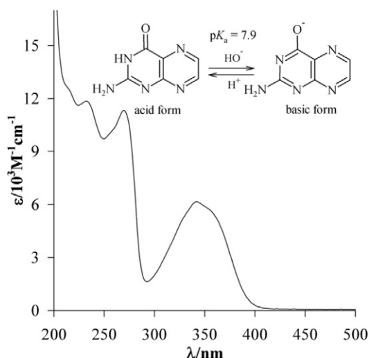
Fig. 1. Molecular structure of Ptr and the absorption spectra in buffer Tris pH 7.4.
