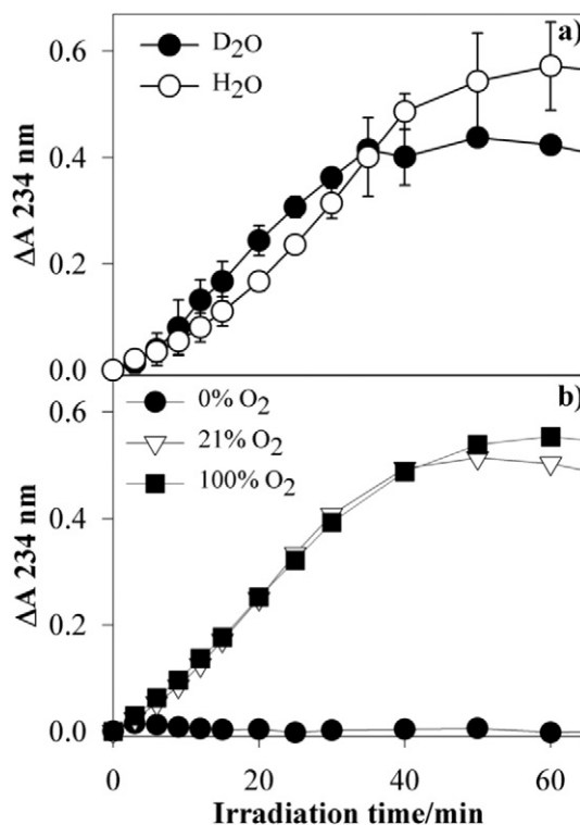
Fig. 5. Time evolution of absorbance of conjugated dienes (A234) for liposomes with Ptr as a function of irradiation time under different conditions. a) Experiments carried out in \text{H}_2\text{O} and \text{D}_2\text{O} ; b) experiments carried out in air-equilibrated (21% \text{O}_2 ), \text{O}_2 -saturated (100% \text{O}_2 ) and Ar-bubbled (0% \text{O}_2 ) liposome suspension. Error bars correspond to SD from 2 to 3 different experiments.
