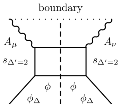
Figure 4. Witten diagram corresponding to the one-loop dominant contribution to FCS.
