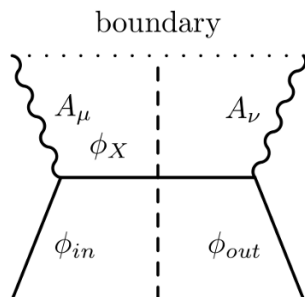
Figure 2. Witten diagram representing the s -channel contribution to the holographic dual description of FCS in the N \rightarrow \infty limit. The vertical dashed line schematically represents the optical theorem procedure used to extract the relevant imaginary part of T^{\mu\nu} . There is a single-hadron intermediate state, which means that only single-hadron final states are considered in DIS. The horizontal dotted line represents the boundary of \text{AdS}_5 . In addition, \phi_{in} , \phi_X and \phi_{out} are the dual supergravity fields of the initial, intermediate and final hadronic states, respectively, while A_\mu couples to J^\mu of the quantum field theory at the AdS boundary.
