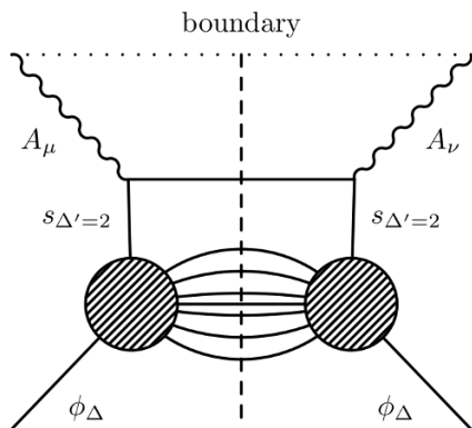
Figure 6. Relevant Witten diagrams at a generic loop-level.
