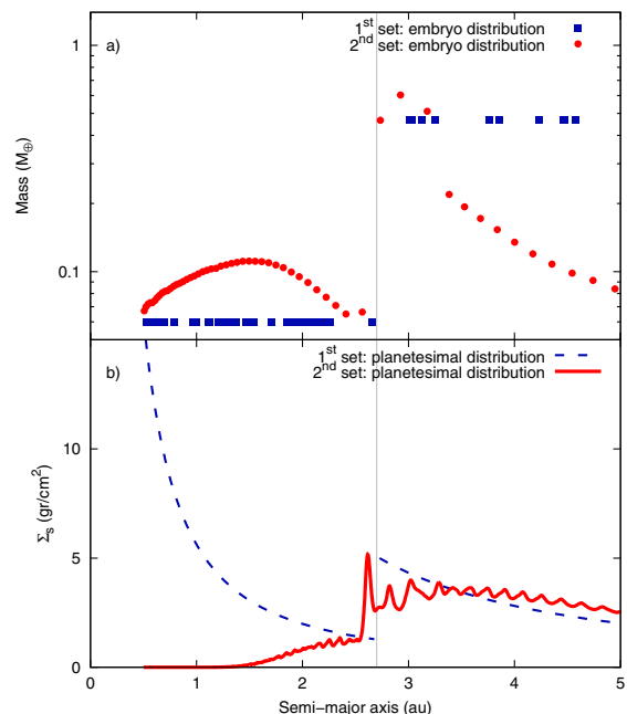
Fig. 2. a) Distributions of embryos used to start the N -body simulations. The squares represent the distribution of embryos obtained with the first set of simulations. The circles represent the final results obtained with the semi-analytical model (the second set of simulations). b) Surface density profiles used to distribute 1000 planetesimals to start the N -body simulations. The dashed line represents the surface density for the first set, the solid line the surface density for the second set obtained with the semi-analytical model. A color figure is available in the electronic version.
