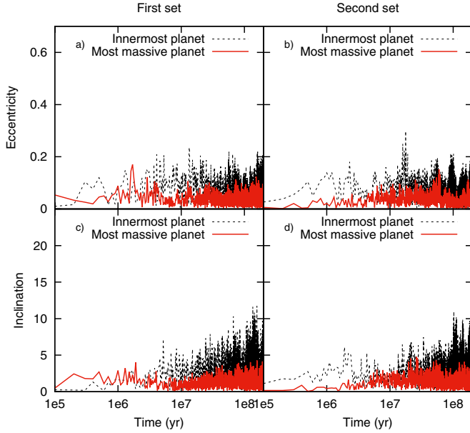
Fig. 6. Evolutions of eccentricities, a), b), and inclinations, c), d), as a function of time for the innermost planet (black curve) and the most massive planet (red curve) of the S3 simulations and S3 simulations in the first and in the second set. The dynamical friction effects prevail over the larger bodies, which evolve in both sets of simulations in regions of the disk that are embedded in a swarm of planetesimals. A color figure is available in the electronic version.
