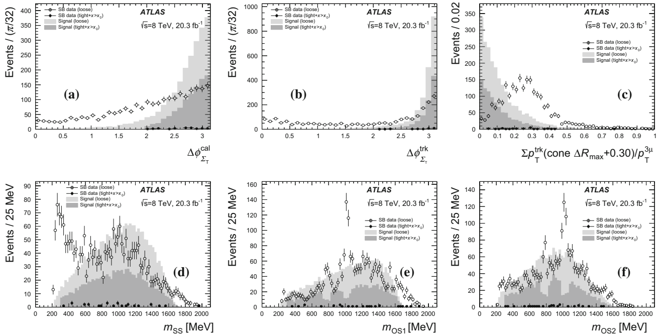
Fig. 4 The complementary variables used in the loose or tight selection but not as inputs for the BDT. \Delta\phi_{\Sigma_T}^{cal} in a , \Delta\phi_{\Sigma_T}^{trk} in b , \Sigma p_T^{trk} (\Delta R_{max}^{3\mu} + 0.30) / p_T^{3\mu} in c , m_{SS} in d , m_{OS1} in e and m_{OS2} in f . The loose data in the sidebands are shown as hollow circles , while the loose signal MC events are shown as light solid grey area . The tight+x>x 0 data in the sidebands are shown as the solid black circles , while the tight+x>x 0 signal
