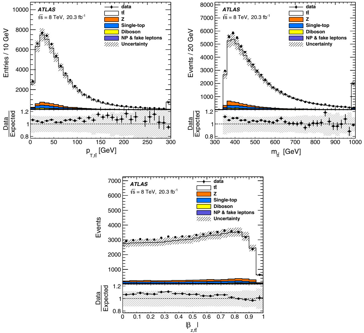
FIG. 2. Distributions of p_{T,\bar{t}t} , m_{\bar{t}t} , and |\beta_{z,\bar{t}t}| for data (points) and predictions (histograms) after kinematic reconstruction. The data/expected ratio is also shown. The shaded area corresponds to the detector systematic uncertainty, the signal modeling systematic uncertainty, and the normalization uncertainty in signal and background. In the p_{T,\bar{t}t} and m_{\bar{t}t} distributions, the last bin includes the overflow.
