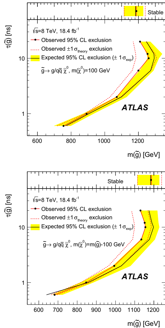
Fig. 7 The excluded range of lifetimes as a function of gluino mass for gluino R -hadrons decaying into g/q\bar{q} plus a light neutralino of mass m(\tilde{\chi}_1^0) = 100\text{ GeV} (top) or a heavy neutralino of mass m(\tilde{\chi}_1^0) = m(\tilde{g}) - 100\text{ GeV} (bottom). The expected exclusion, with its experimental \pm 1\sigma band, is given with respect to the nominal theoretical cross section
