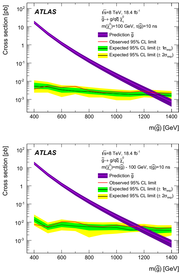
Fig. 6 Upper limits on the production cross section as a function of mass for metastable gluino R -hadrons, with lifetime \tau = 10\text{ ns} , decaying into g/q\bar{q} plus a light neutralino of mass m(\tilde{\chi}_1^0) = 100\text{ GeV} (top) or a heavy neutralino of mass m(\tilde{\chi}_1^0) = m(\tilde{g}) - 100\text{ GeV} (bottom). Theoretical values for the cross section are shown with their uncertainty. The expected upper limit in the background-only case is shown as a solid black line, with its \pm 1\sigma and \pm 2\sigma bands, green and yellow, respectively. The observed 95% CL upper limit is shown as a solid red line
