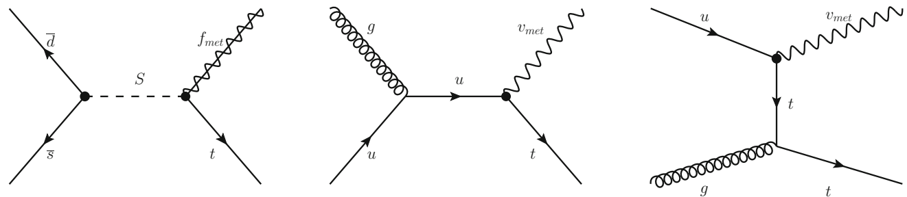
Fig. 1 Example of Feynman diagrams of leading-order processes leading to monotop events: ( left ) production of a coloured scalar resonance S decaying into a top quark and a spin-1/2 fermion f_{\text{met}} in the resonant
