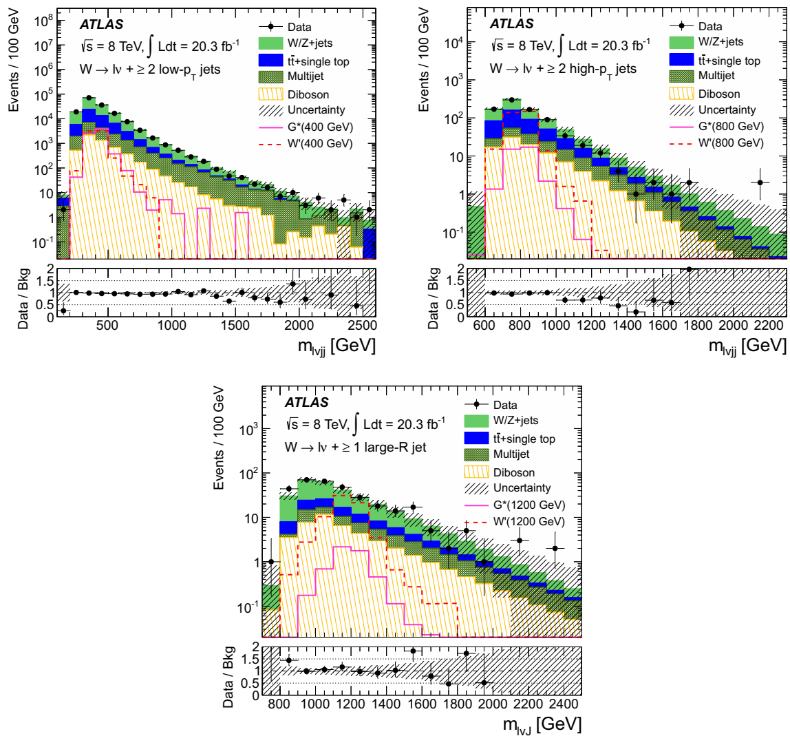
Fig. 1 Reconstructed mass distributions in data and the predicted backgrounds in the three kinematic regions referred to in the text as the low- p_T resolved region (top left), high- p_T resolved region (top right) and merged region (bottom). G^* and W' signal hypotheses of masses 400,
