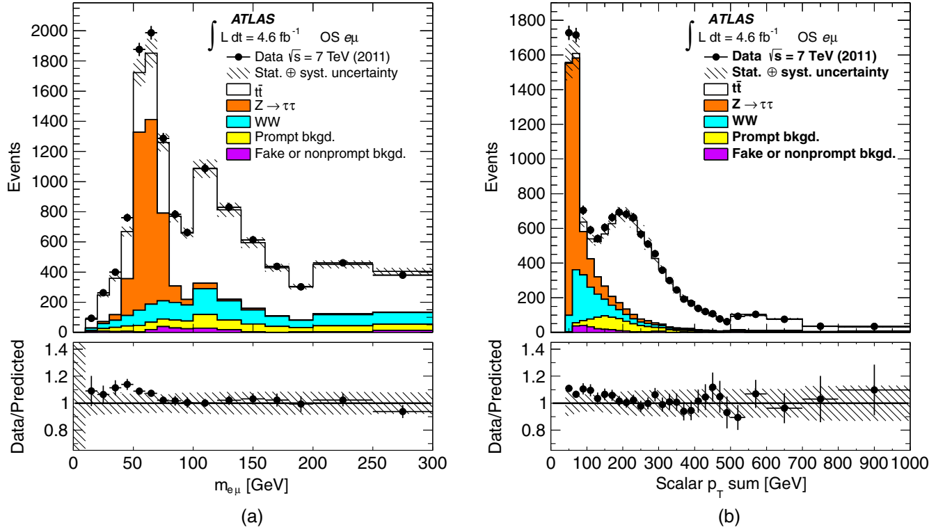
FIG. 2 (color online). Comparison between data and Monte Carlo samples (including the data-driven fake described in Sec. V and nonprompt backgrounds described in Sec. III) normalized to their theoretical cross-sections for an integrated luminosity of 4.6 \text{ fb}^{-1} : (a) invariant mass distribution of electron and muon pairs and (b) distribution of the scalar sum of the transverse momenta of the selected electron, muon and jets. The electron and muon of OS charge satisfy the signal region selection criteria presented in Sec. IV. A bin by bin ratio between the data and simulated events is shown at the bottom of each comparison. The hatched regions represent the combination of statistical and systematic uncertainties as listed in Table II (except for shape uncertainties) and described in Sec. VI together with the full theoretical cross-section uncertainties for the t\bar{t} , WW , and Z/\gamma^* \rightarrow \tau\tau signal processes.
