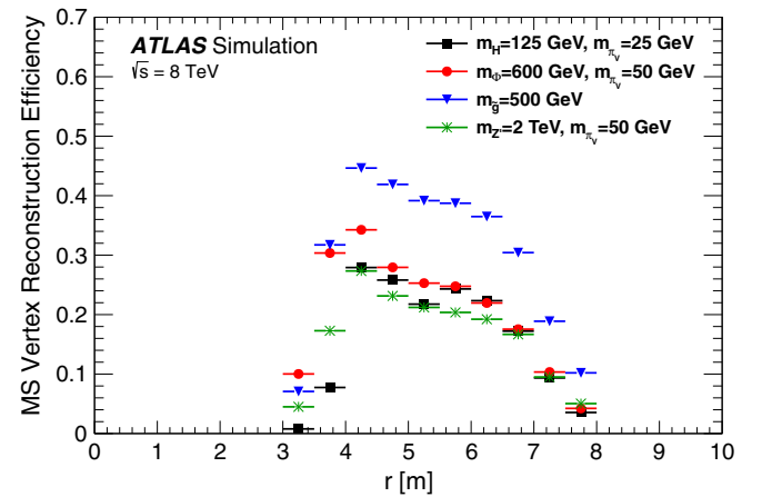
FIG. 7 (color online). Barrel MS vertex reconstruction efficiency as a function of the radial decay position of the long-lived particle for scalar boson, Stealth SUSY, and Z' benchmark samples.
