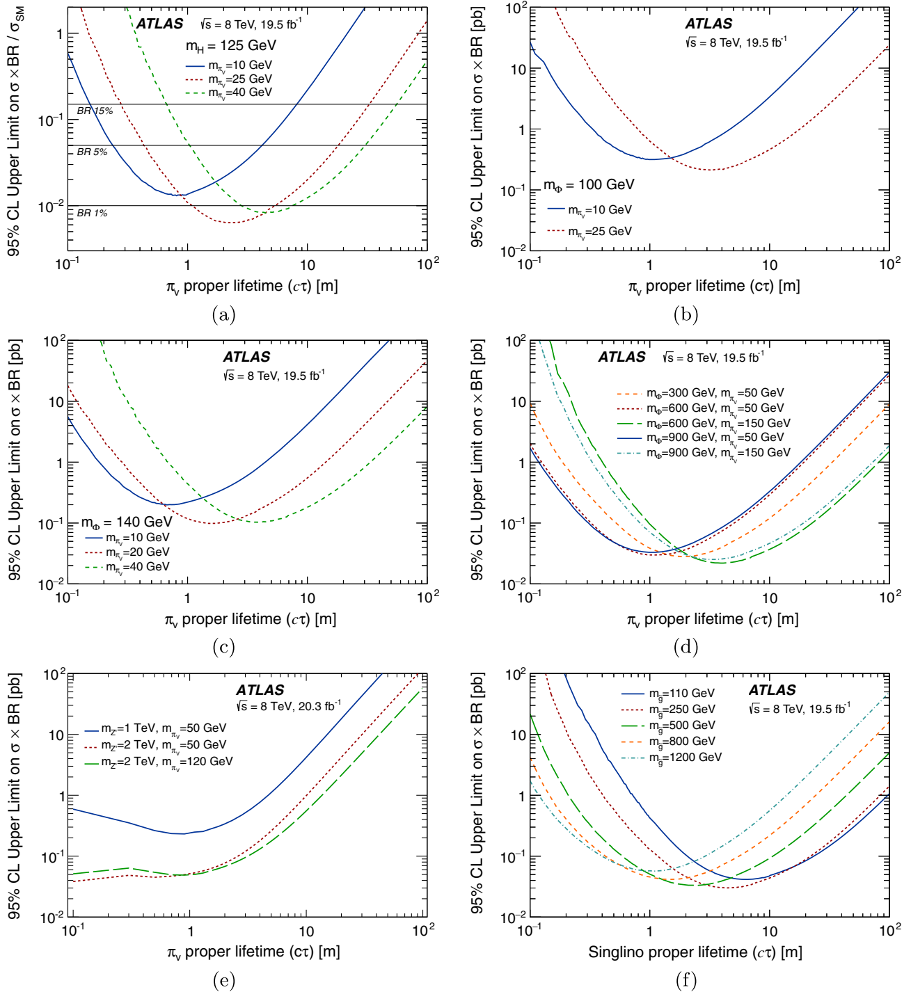
FIG. 10 (color online). (a) Observed 95% C.L. limits on \sigma \times \text{BR} / \sigma_{\text{SM}} for the scalar boson samples with m_H = 125 GeV. Three horizontal lines mark branching fractions for the Higgs boson decaying to \pi_\nu pairs at 15%, 5%, and 1%. Observed 95% C.L. limits on \sigma \times \text{BR} for the scalar boson samples with (b) m_\phi = 100 GeV, (c) m_\phi = 140 GeV, and (d) m_\phi = 300, 600, and 900 GeV. Observed 95% C.L. limits on \sigma \times \text{BR} for the (e) Z' samples and (f) Stealth SUSY samples.
