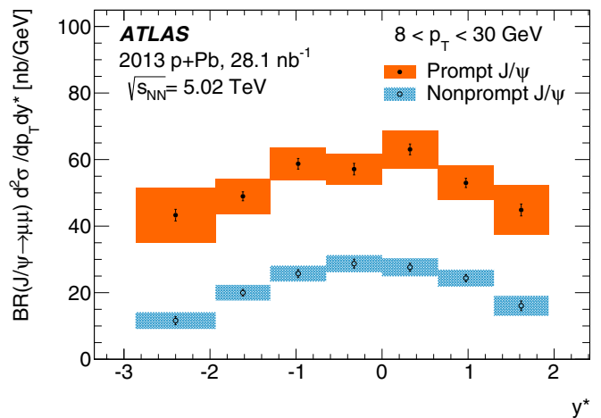
FIG. 5. (Color online) Double differential cross section for prompt and nonprompt J/\psi as a function of J/\psi c.m. rapidity y^* . Positive y^* is defined in the proton beam direction. The error bars show the statistical uncertainty, and the shaded boxes show the sum in quadrature of statistical and systematic uncertainties.
