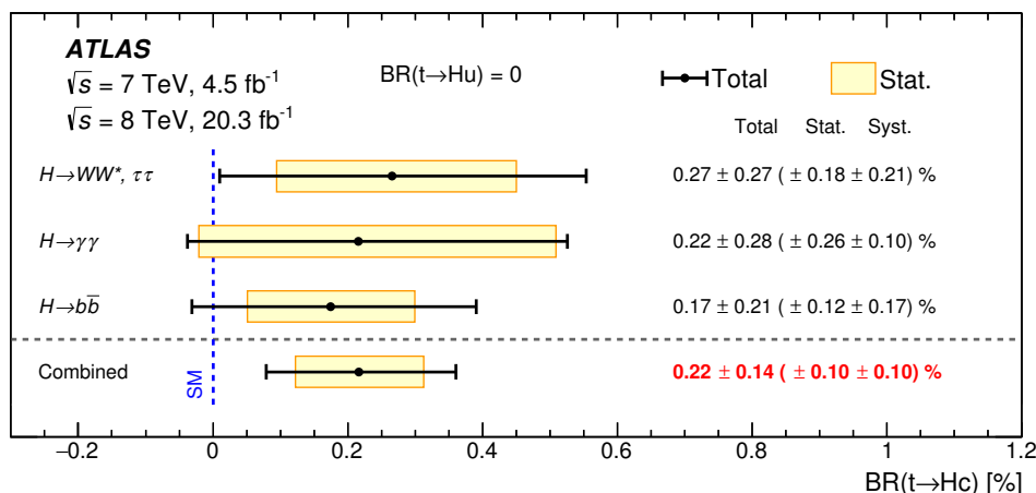
Figure 9. Summary of the best-fit BR(t \rightarrow Hc) for the individual searches as well as their combination, assuming that BR(t \rightarrow Hu) = 0 .
