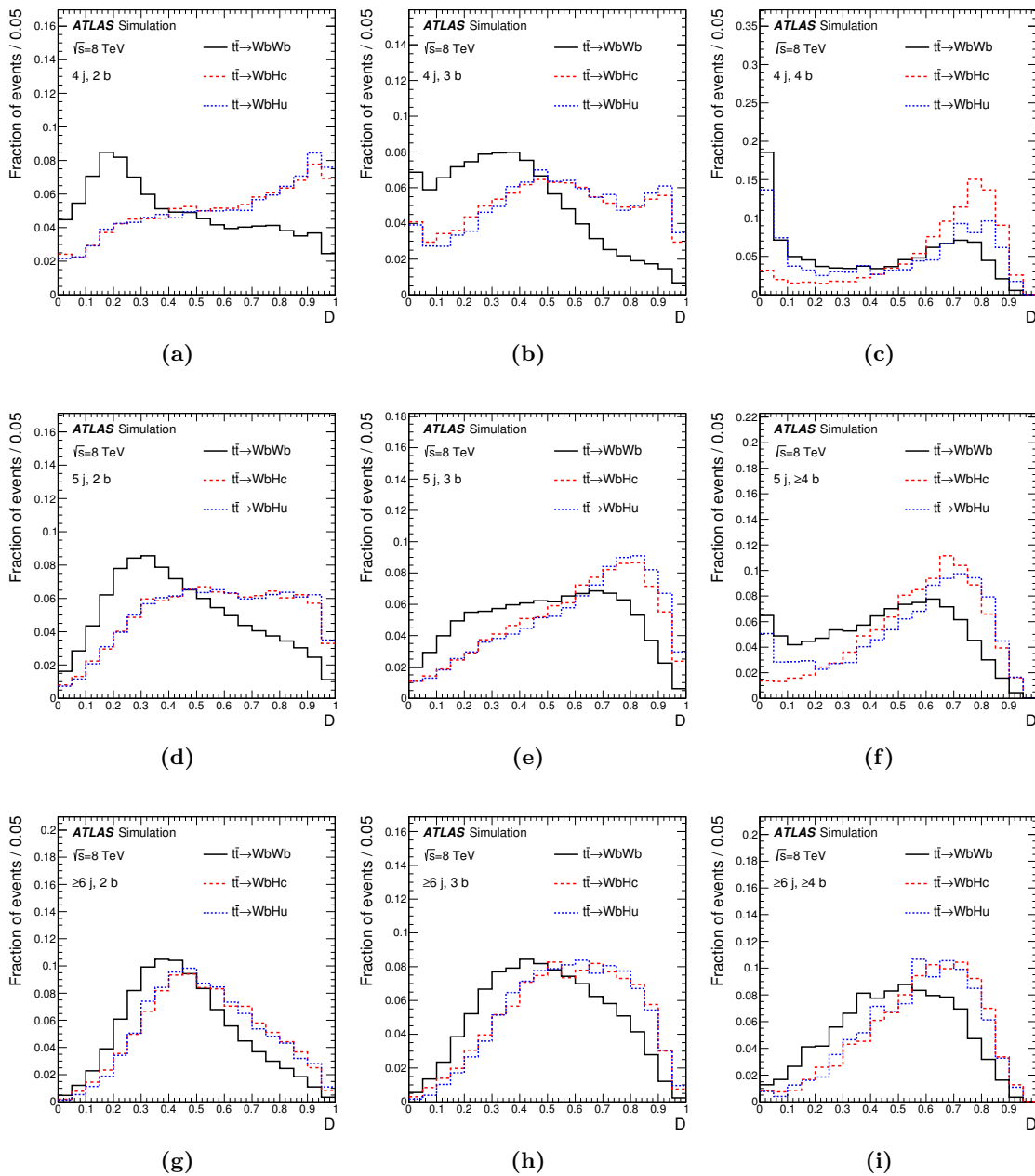
Figure 3. Comparison of the shape of the D discriminant distribution between the t\bar{t} \rightarrow WbHc (red dashed) and t\bar{t} \rightarrow WbHu (blue dotted) signals, and the t\bar{t} \rightarrow WbWb background (black solid) in each of the channels considered in the analysis: (a) (4 j, 2 b), (b) (4 j, 3 b), (c) (4 j, 4 b), (d) (5 j, 2 b), (e) (5 j, 3 b), (f) (5 j, \geq 4 b), (g) ( \geq 6 j, 2 b), (h) ( \geq 6 j, 3 b), and (i) ( \geq 6 j, \geq 4 b).
