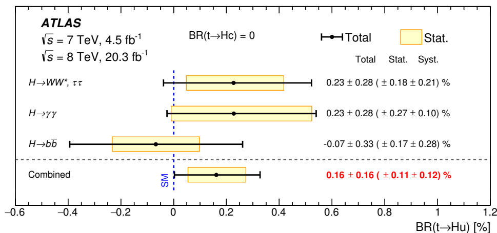
Figure 10. Summary of the best-fit BR(t \rightarrow Hu) for the individual searches as well as their combination, assuming that BR(t \rightarrow Hc) = 0 .
