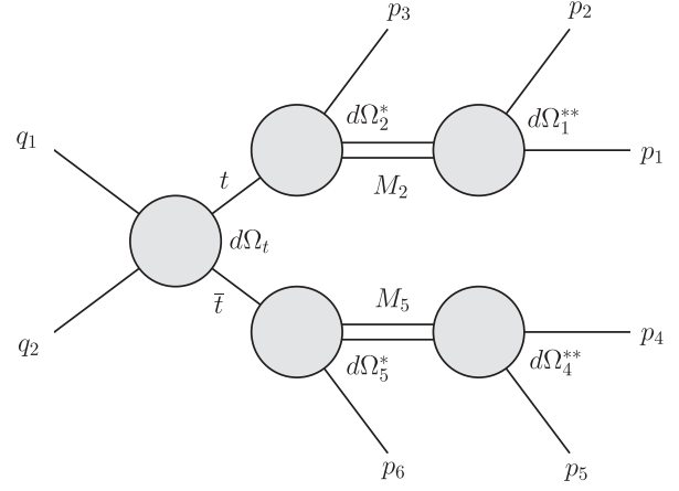
FIG. 1. Kinematics for gg \rightarrow t\bar{t} \rightarrow (b\bar{b}c)(\bar{b}\ell\bar{\nu}) [10]. The definitions of the various angles and invariant masses are identical to those given in Ref. [7]; these definitions are reproduced here for convenience. \Omega_1^{**} denotes the direction of \vec{p}_1^{**} in the rest frame of M_2 , relative to the direction of \vec{p}_1^* + \vec{p}_2^* , where M_2^2 = (p_1 + p_2)^2 . Similarly, \Omega_2^* denotes the direction of (\vec{p}_1^* + \vec{p}_2^*) in the t rest frame, relative to the direction of \vec{p}_t in the t\bar{t} rest frame. \Omega_t denotes the direction of \vec{p}_t relative to \vec{q}_1 , also in the t\bar{t} rest frame. The solid angles \Omega_4^{**} and \Omega_5^* are defined analogously to \Omega_1^{**} and \Omega_2^* , respectively, and M_5^2 = (p_4 + p_5)^2 . In this work we take p_1 = p_c , p_2 = p_b , p_3 = p_{\bar{b}_1} , p_4 = p_{\bar{\nu}} , p_5 = p_{\bar{b}_2} and p_6 = p_\ell .
