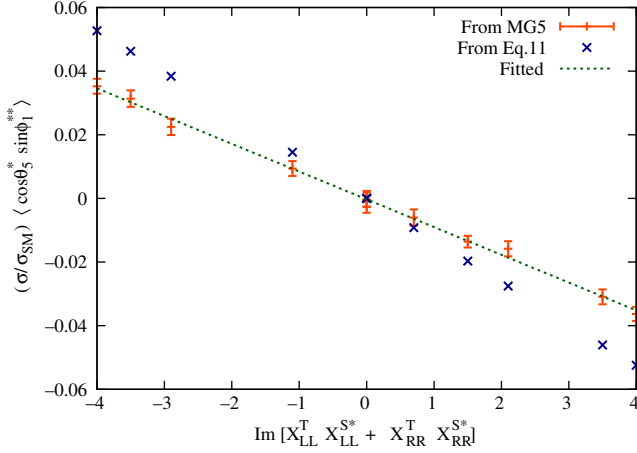
FIG. 2. Plot of (\sigma/\sigma_{\text{SM}})\langle\cos\theta_5^*\sin\phi_1^{**}\rangle as a function of \text{Im}[X_{LL}^T X_{LL}^{S*} + X_{RR}^T X_{RR}^{S*}] for various combinations of NP parameters. As is evident from the plot, the simulated data have a linear dependence on \text{Im}[X_{LL}^T X_{LL}^{S*} + X_{RR}^T X_{RR}^{S*}] , as in Eq. (11), even though Eq. (11) was derived under several simplifying assumptions.
